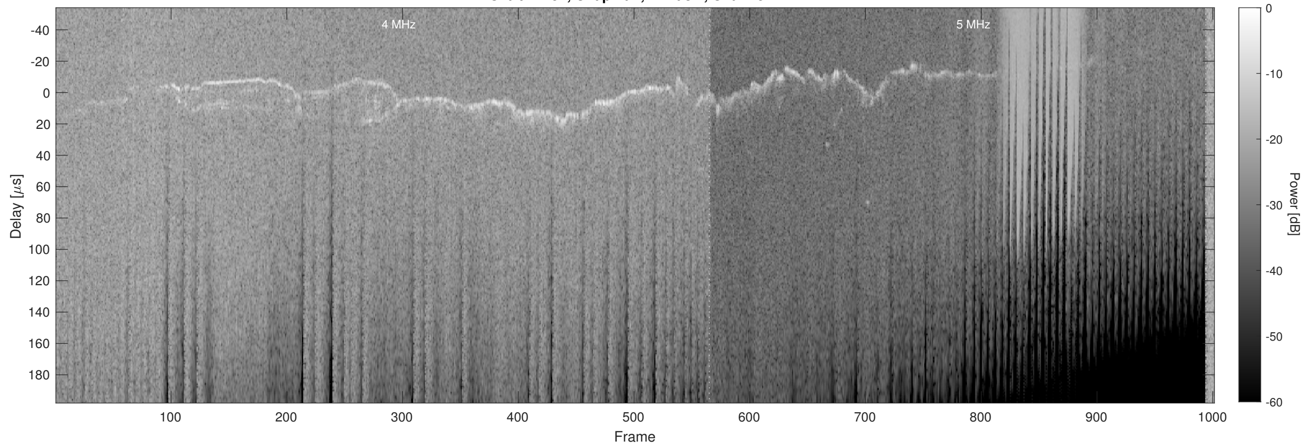
Orbit 12754, Chapman, Window, Channel 2
