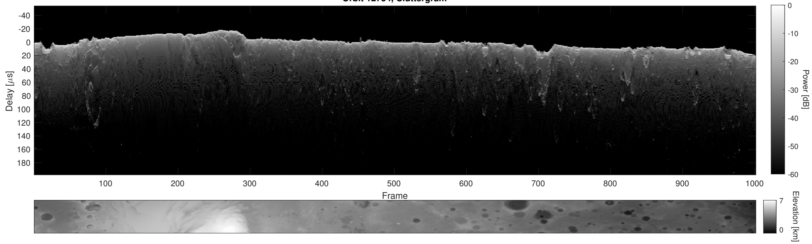
Orbit 12754, Cluttergram
