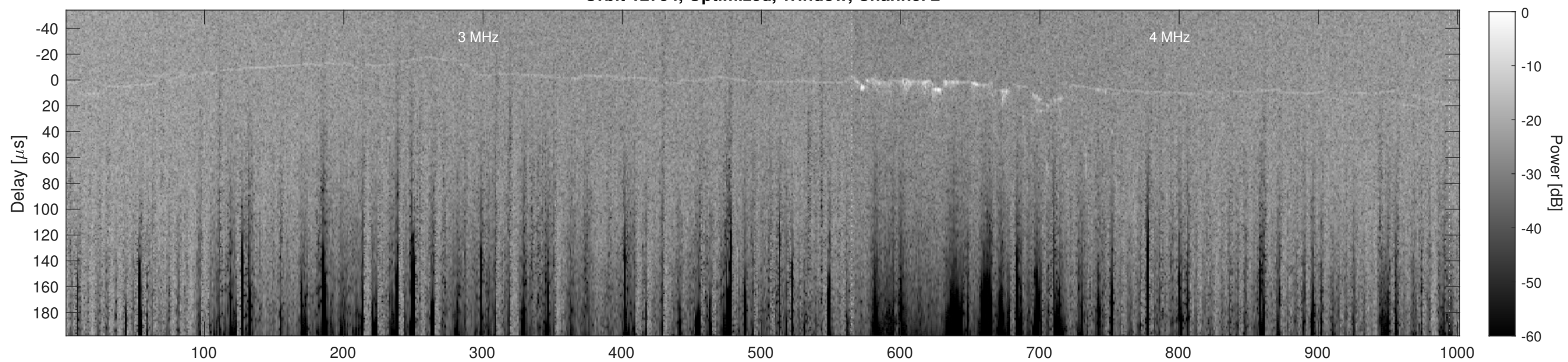
Orbit 12754, Cluttergram
