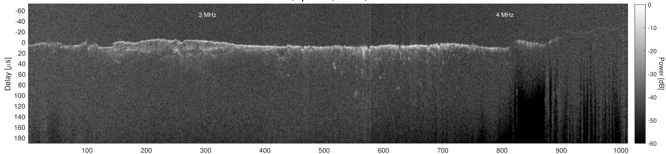
Orbit 12762, Cluttergram
