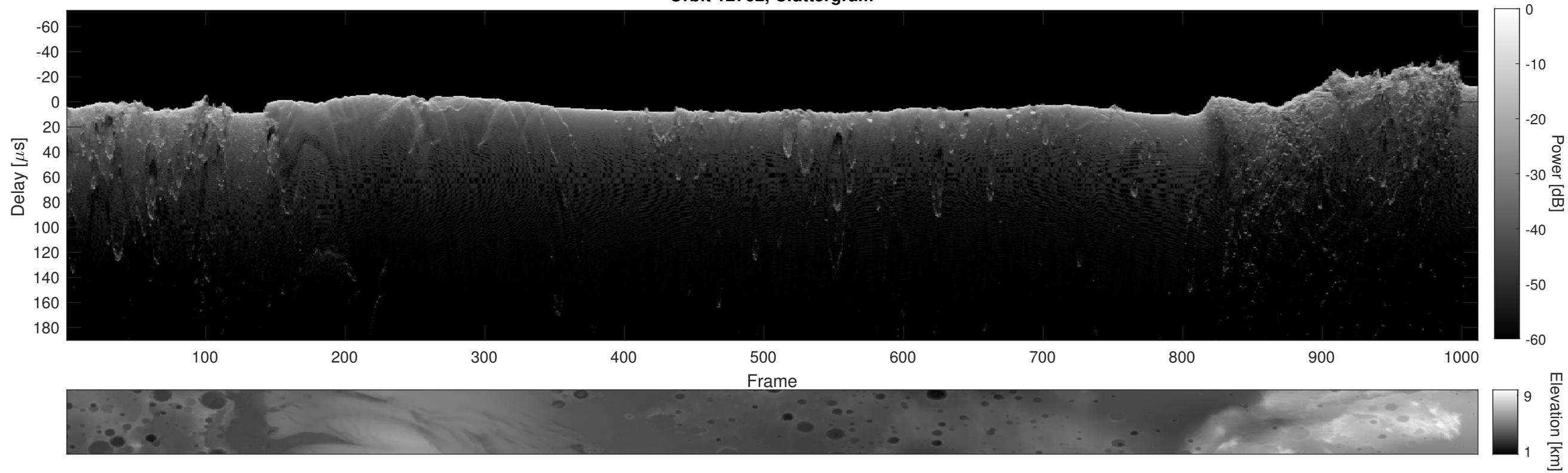
Orbit 12762, Cluttergram
