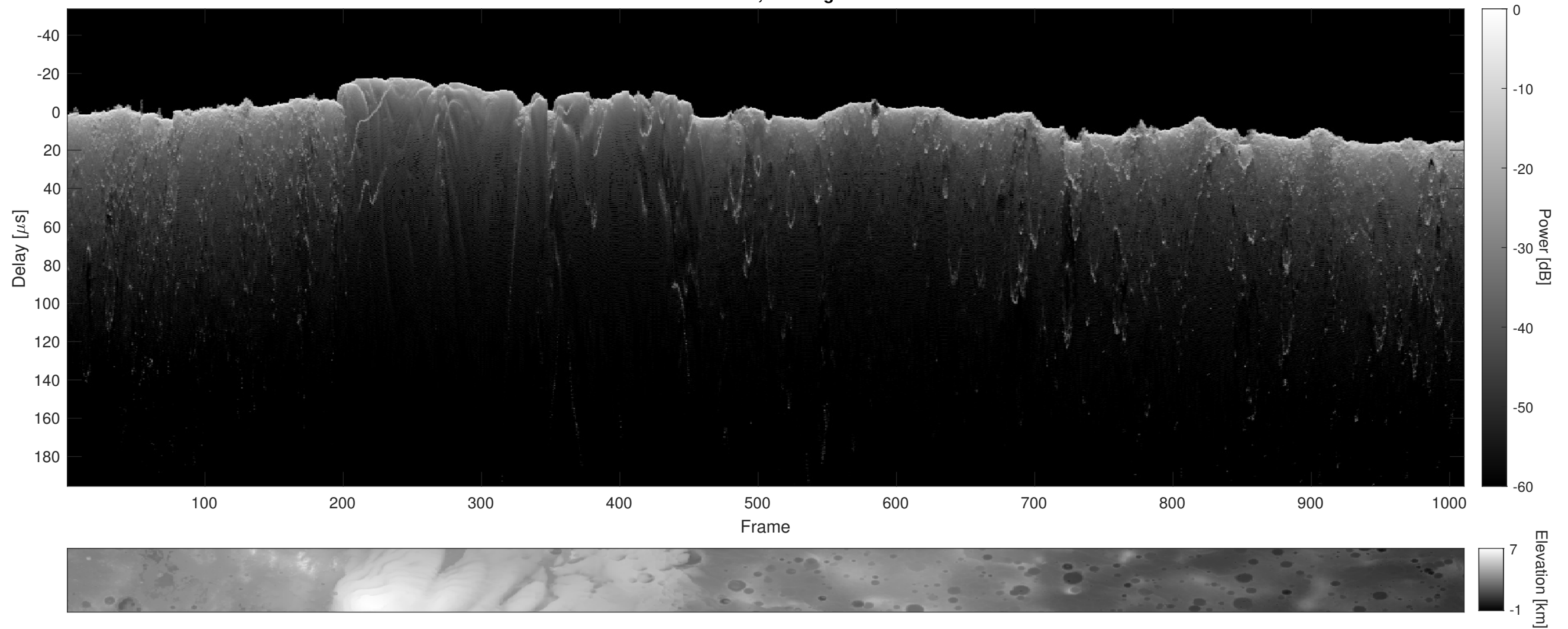
Orbit 12763, Cluttergram
