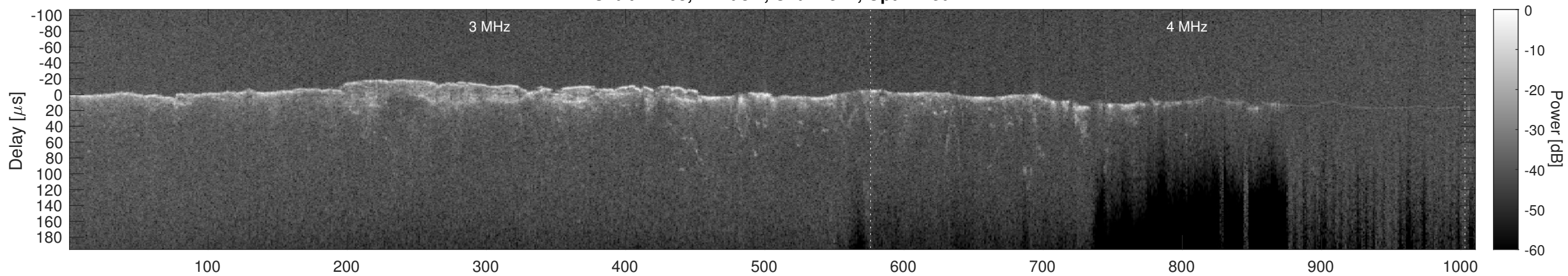
Orbit 12763, Cluttergram
