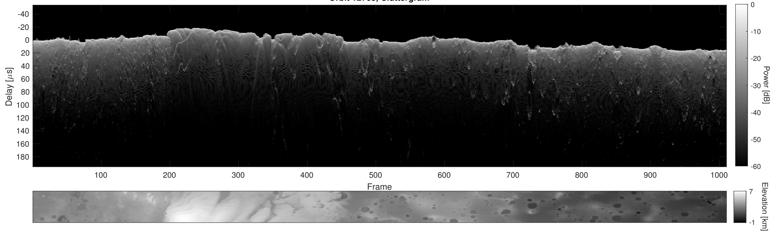
Orbit 12763, Cluttergram
