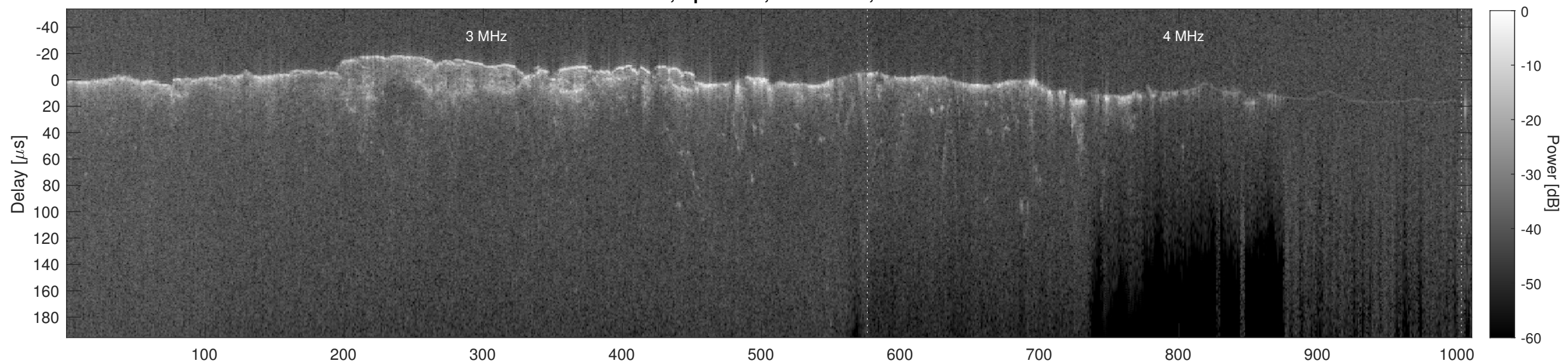
Orbit 12763, Cluttergram
