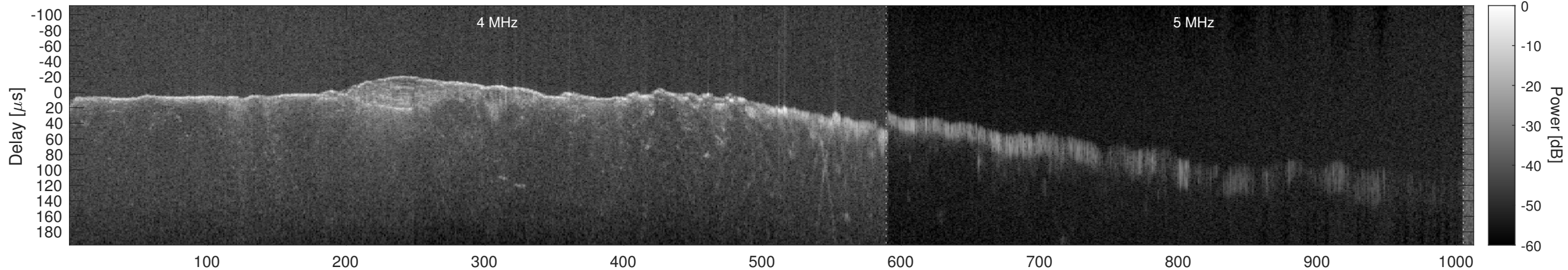
Orbit 12767, Window, Channel 1, Chapman
