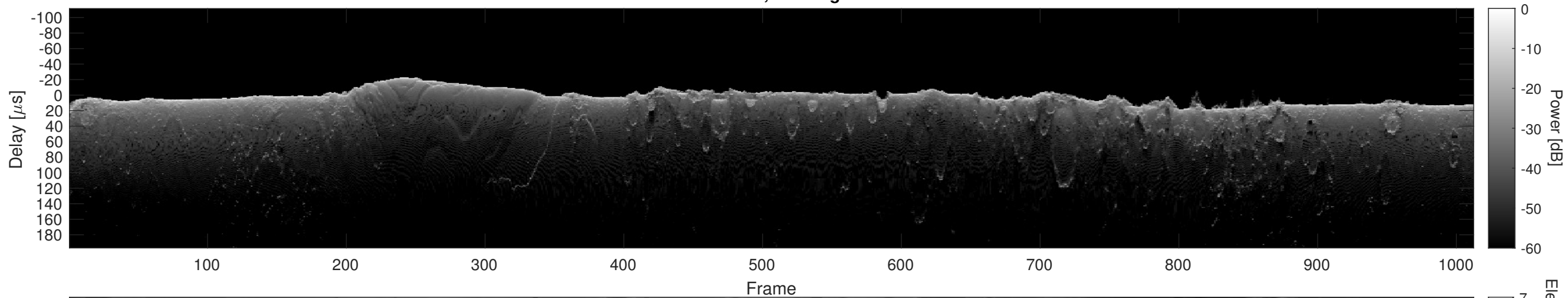
Orbit 12767, Cluttergram
