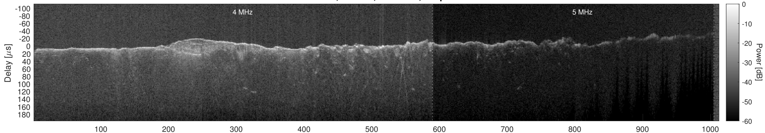
Orbit 12767, Window, Channel 1, Optimized
