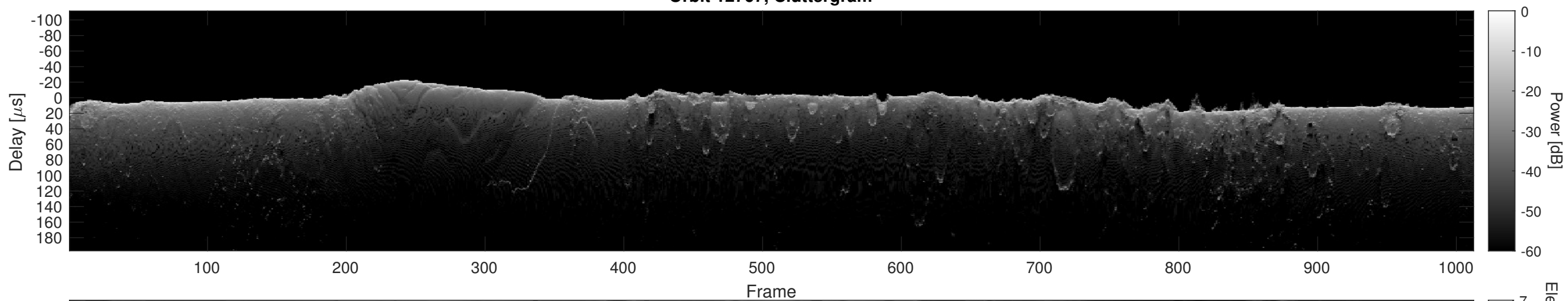
Orbit 12767, Cluttergram
