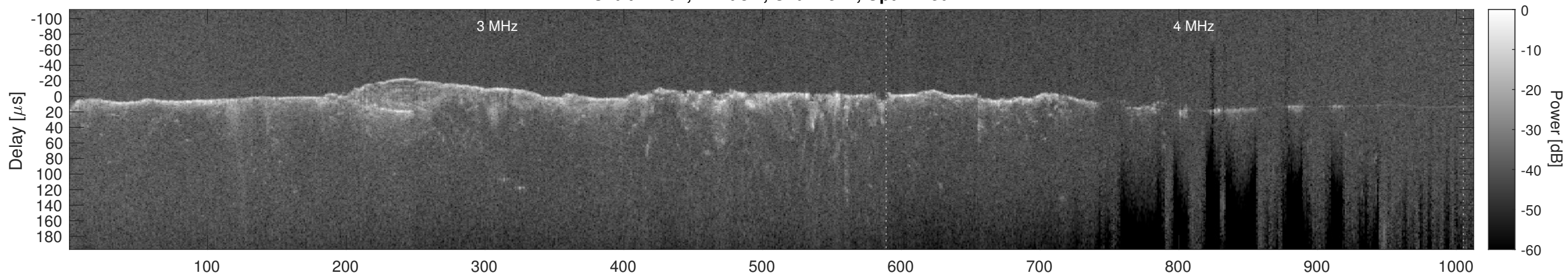
Orbit 12767, Cluttergram
