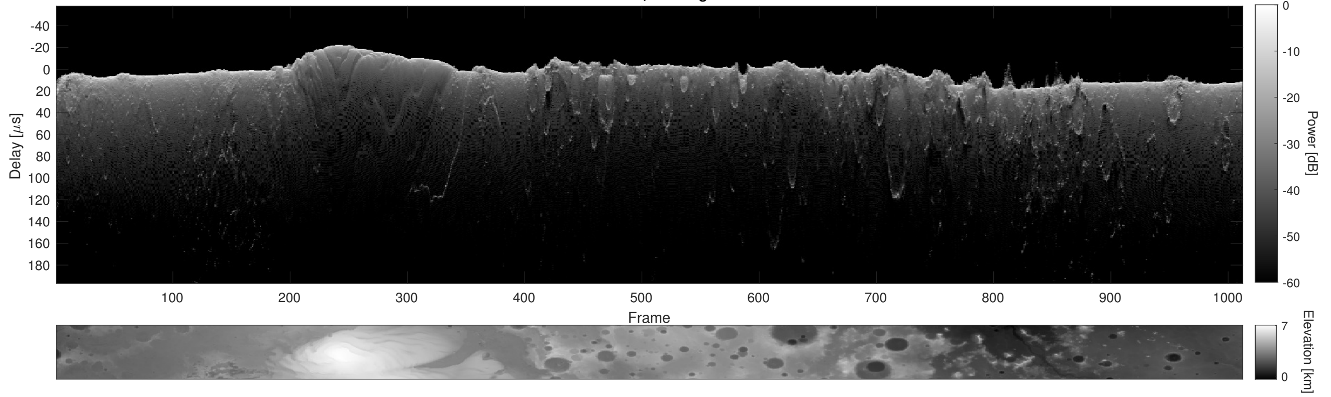
Orbit 12767, Cluttergram
