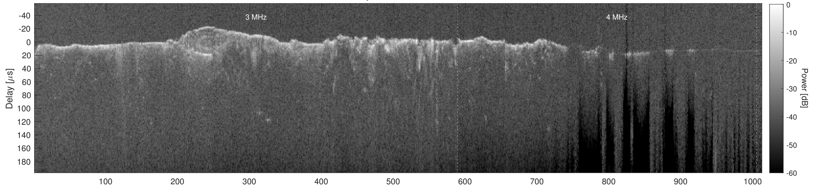
Orbit 12767, Cluttergram
