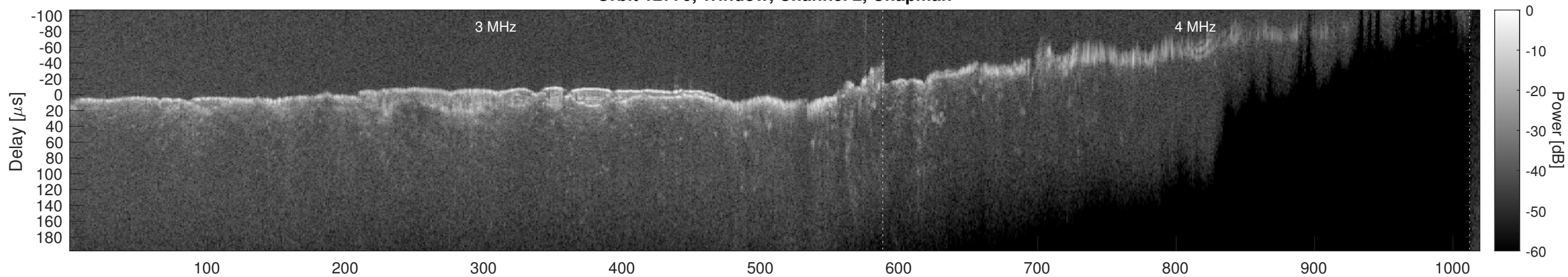
Orbit 12770, Window, Channel 2, Optimized
