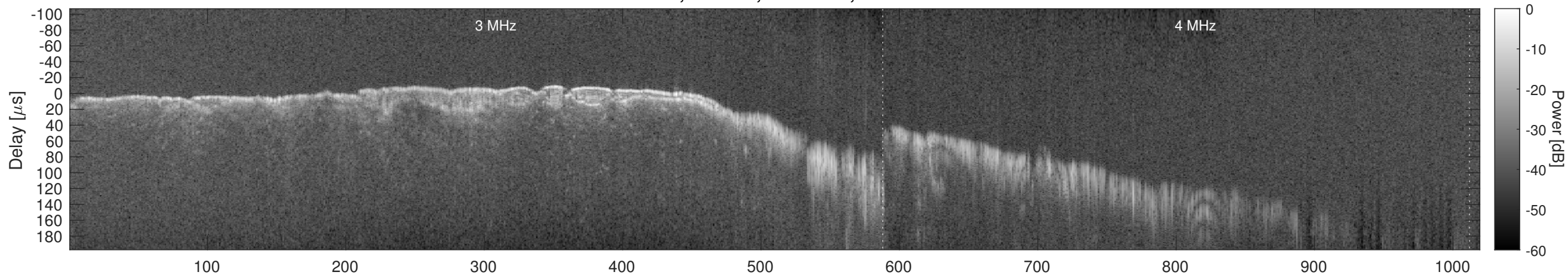
Orbit 12770, Window, Channel 2, Chapman
