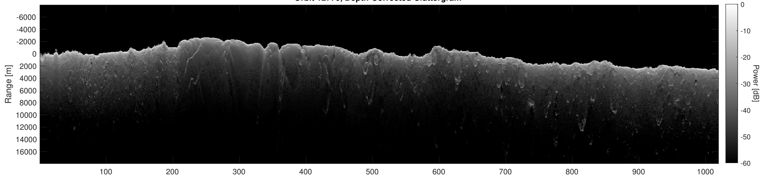
Orbit 12770, Depth-Corrected Cluttergram
