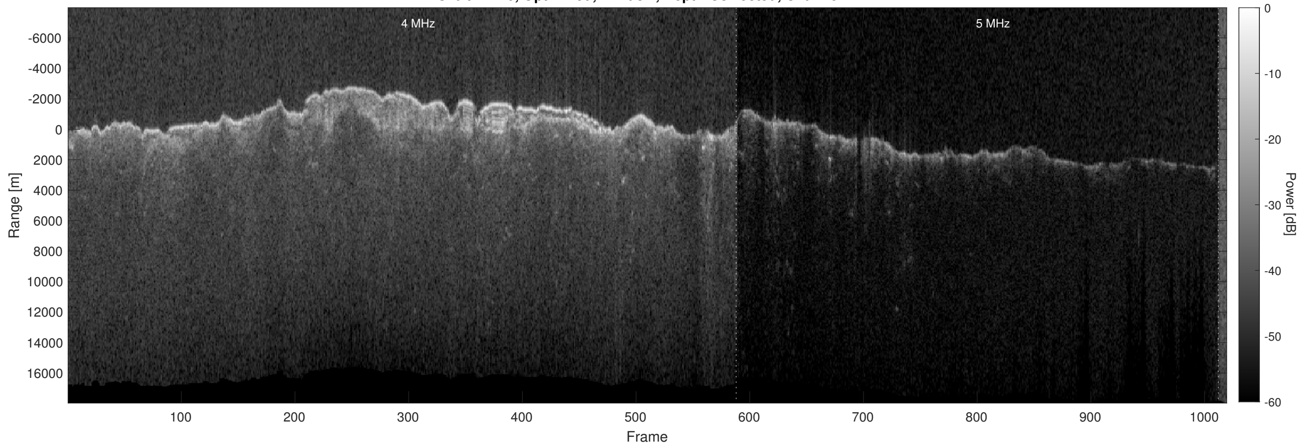
Orbit 12770, Optimized, Window, Depth-Corrected, Channel 2
