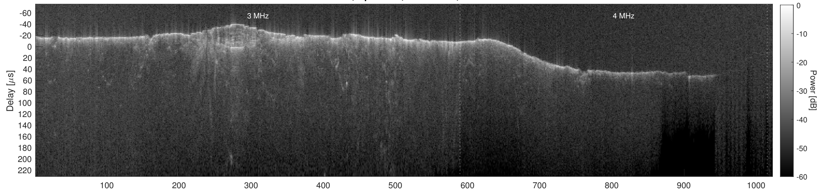
Orbit 12771, Cluttergram
