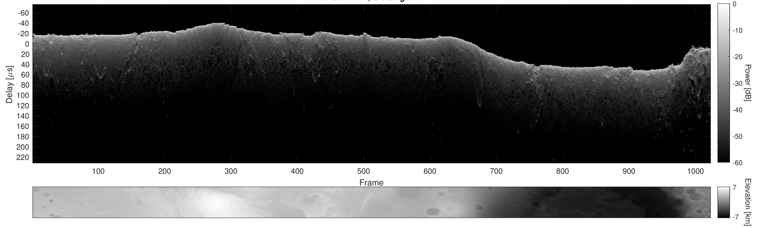
Orbit 12771, Cluttergram
