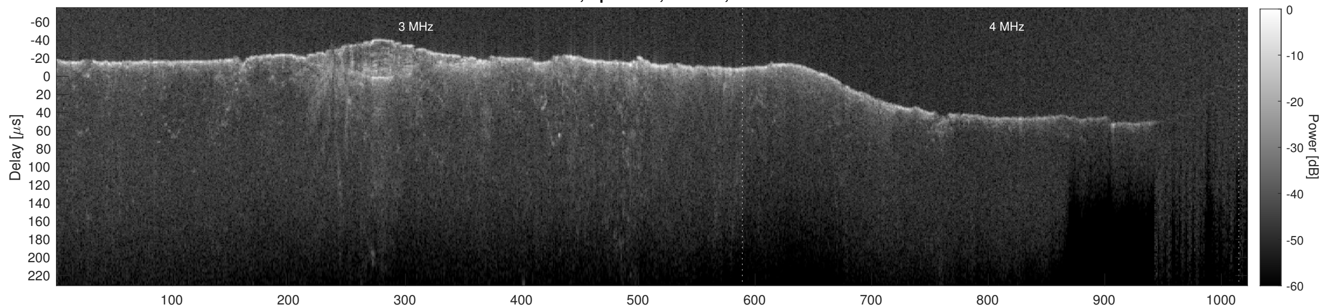
Orbit 12771, Cluttergram
