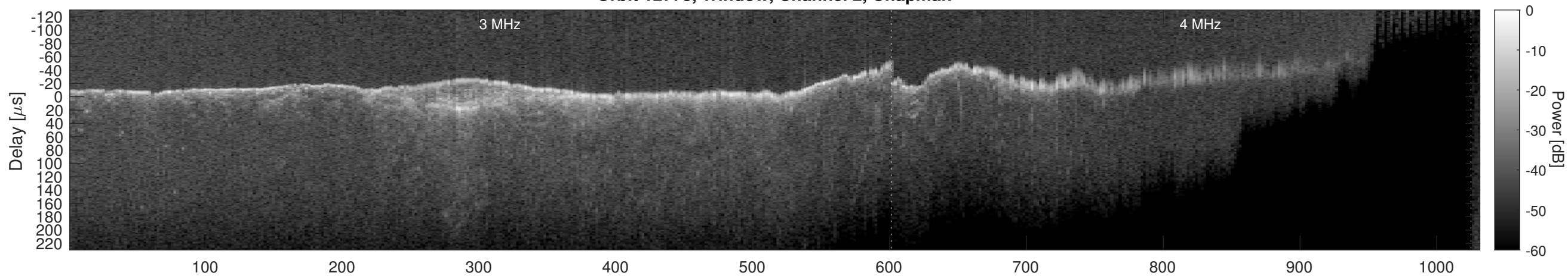
Orbit 12778, Window, Channel 2, Optimized
