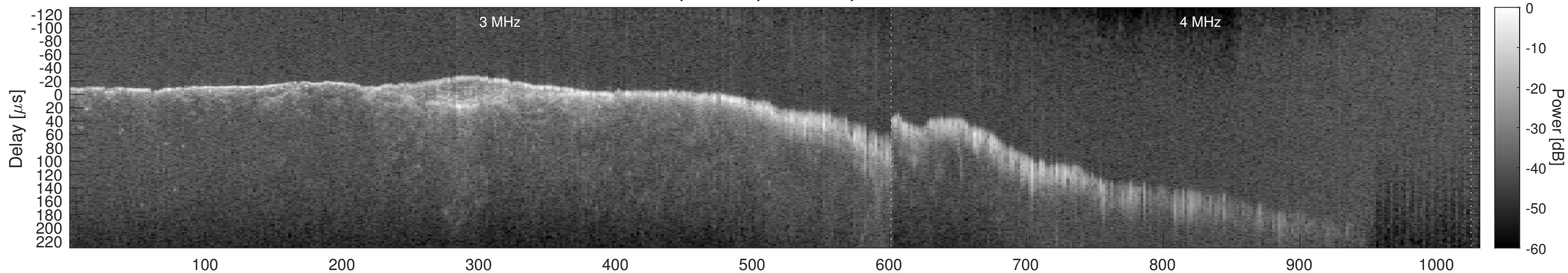
Orbit 12778, Window, Channel 2, Chapman
