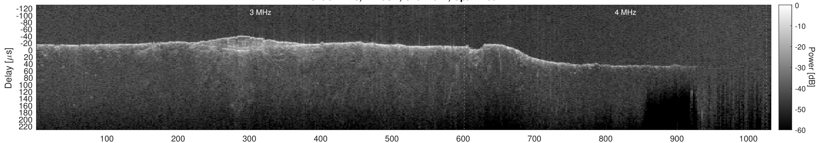
Orbit 12778, Cluttergram
