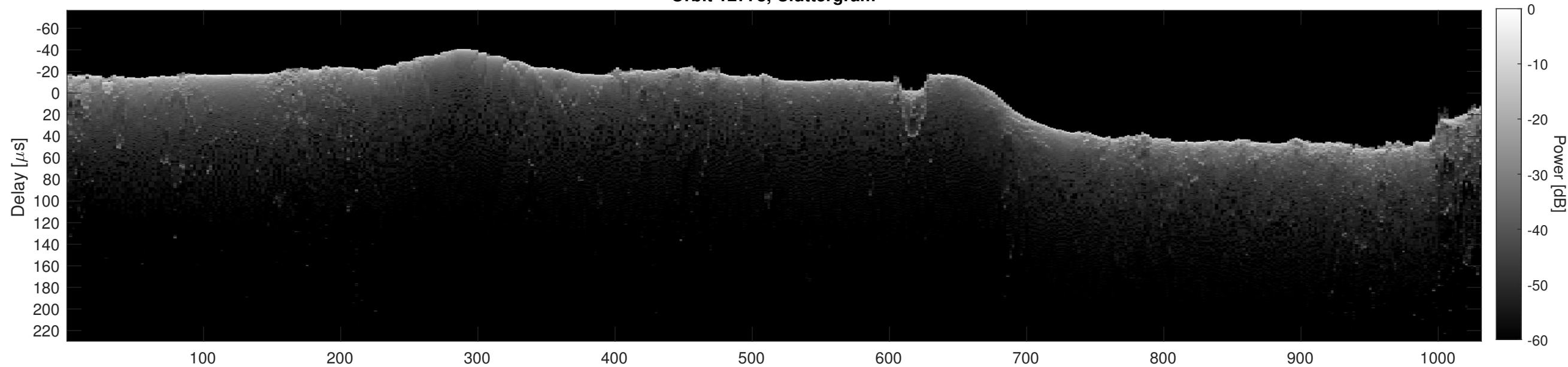
Orbit 12778, Cluttergram
