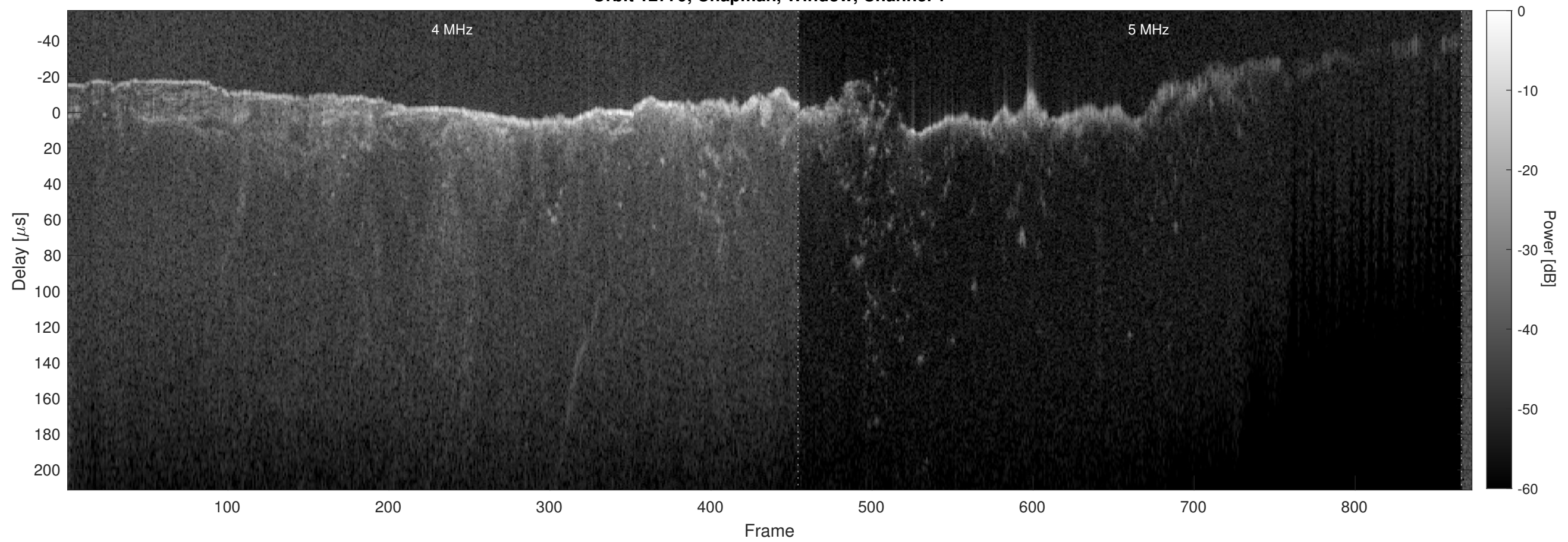
Orbit 12779, Chapman, Window, Channel 2
