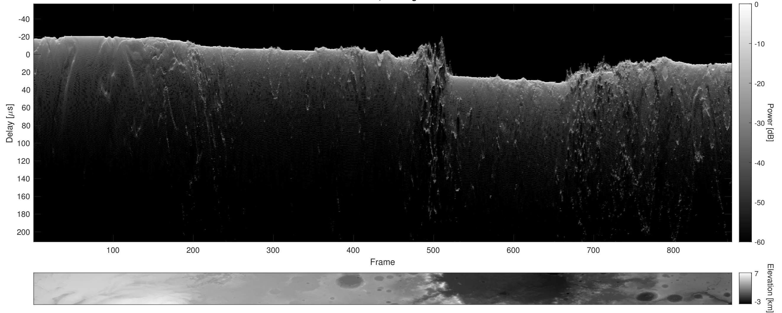
Orbit 12779, Cluttergram
