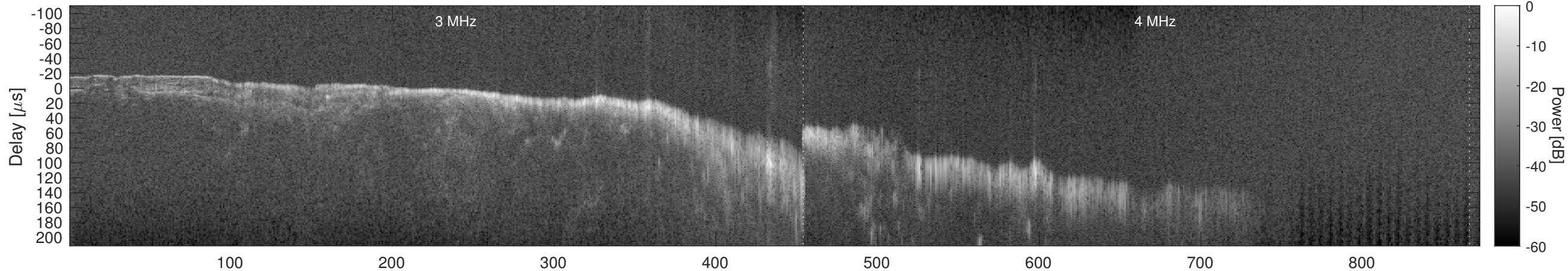
Orbit 12779, Window, Channel 2, Chapman
