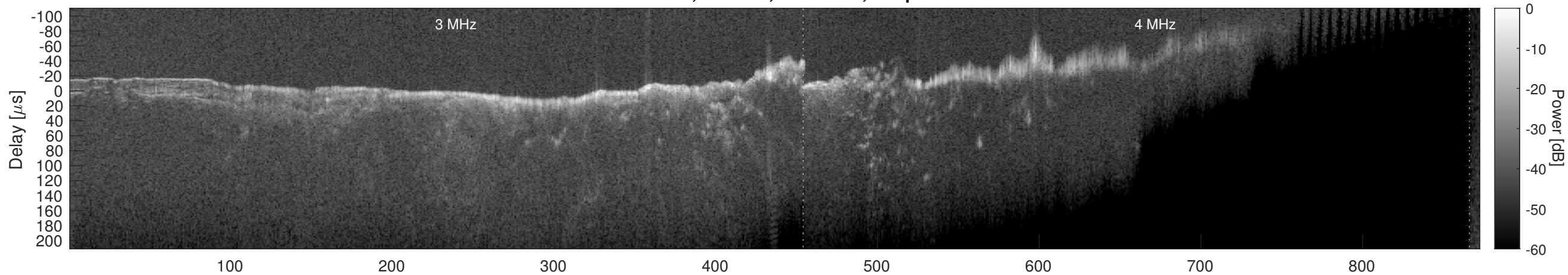
Orbit 12779, Window, Channel 2, Optimized
