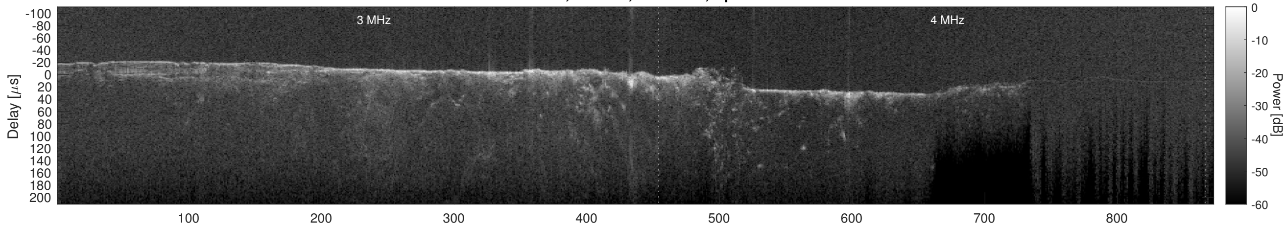
Orbit 12779, Cluttergram
