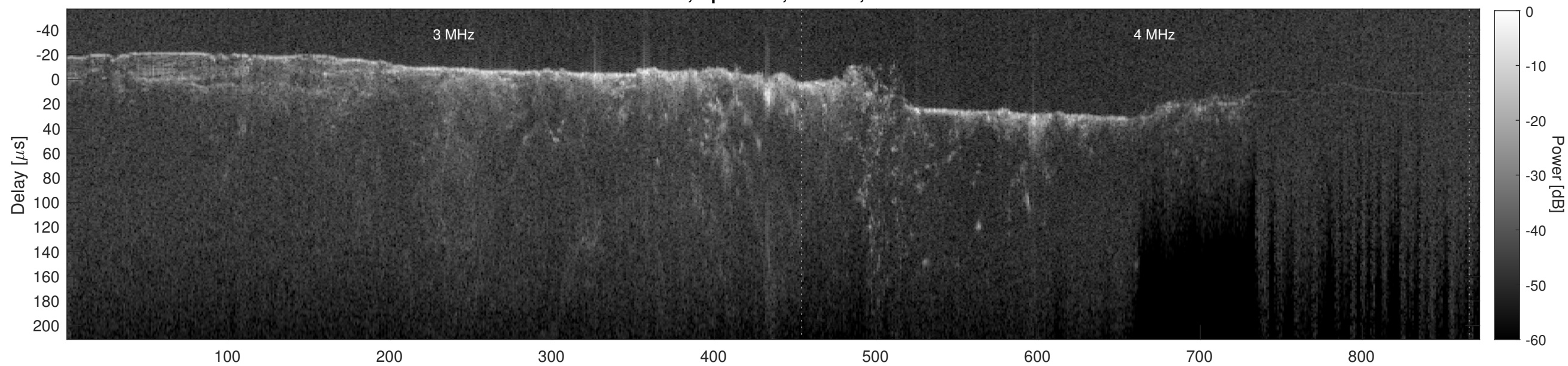
Orbit 12779, Cluttergram
