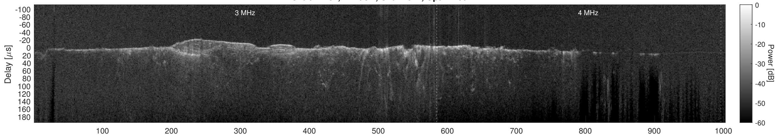
Orbit 12781, Cluttergram
