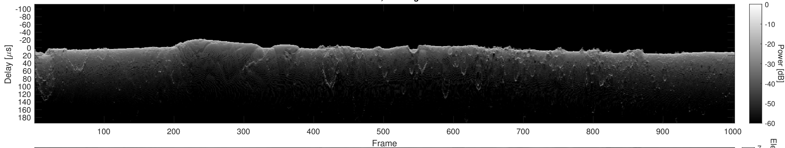
Orbit 12781, Cluttergram
