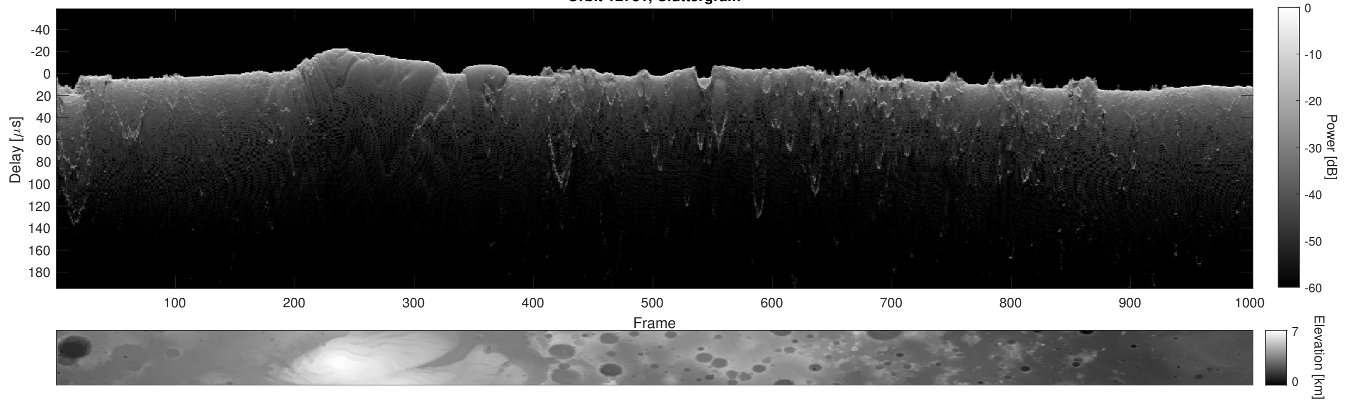
Orbit 12781, Cluttergram
