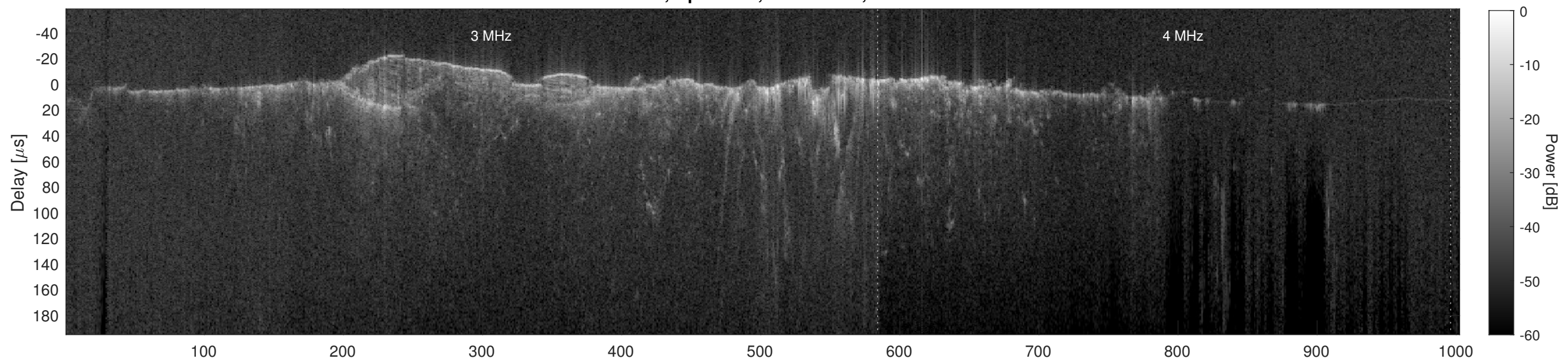
Orbit 12781, Cluttergram
