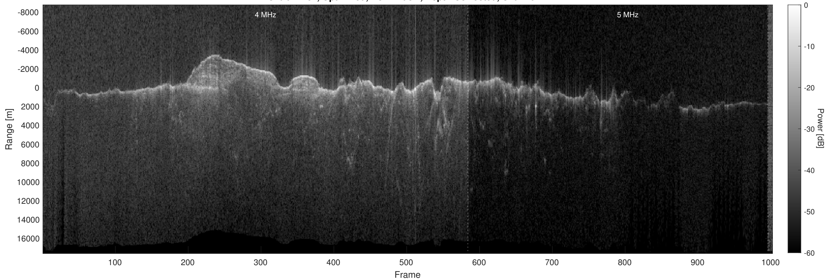
Orbit 12781, Optimized, No Window, Depth-Corrected, Channel 2
