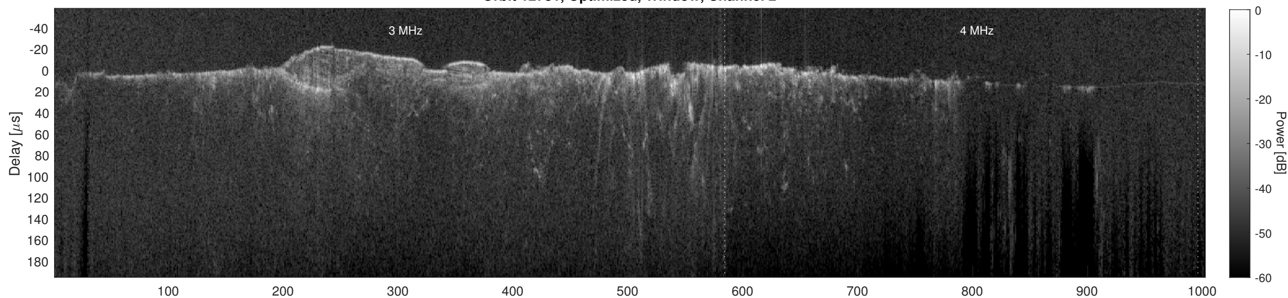
Orbit 12781, Cluttergram
