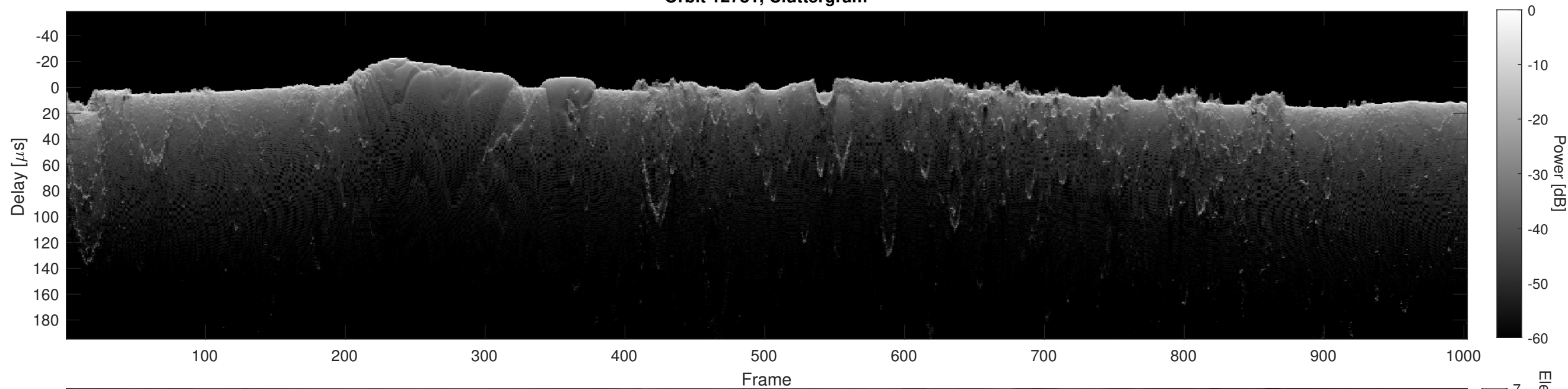
Orbit 12781, Cluttergram
