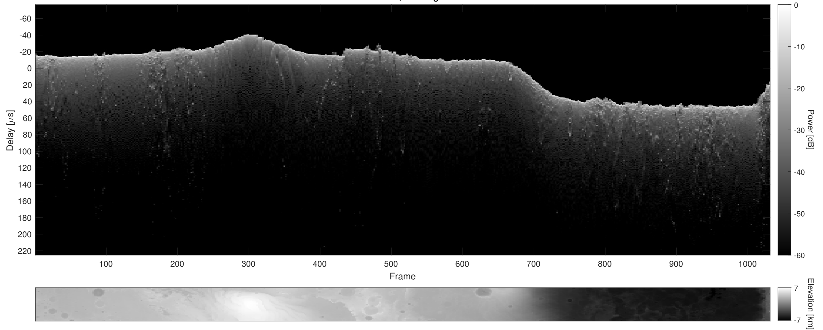
Orbit 12785, Cluttergram
