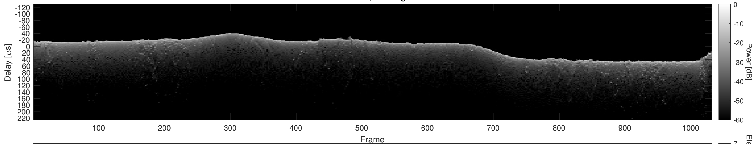
Orbit 12785, Cluttergram
