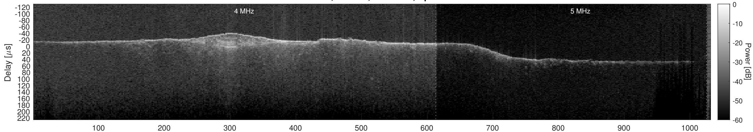
Orbit 12785, Cluttergram
