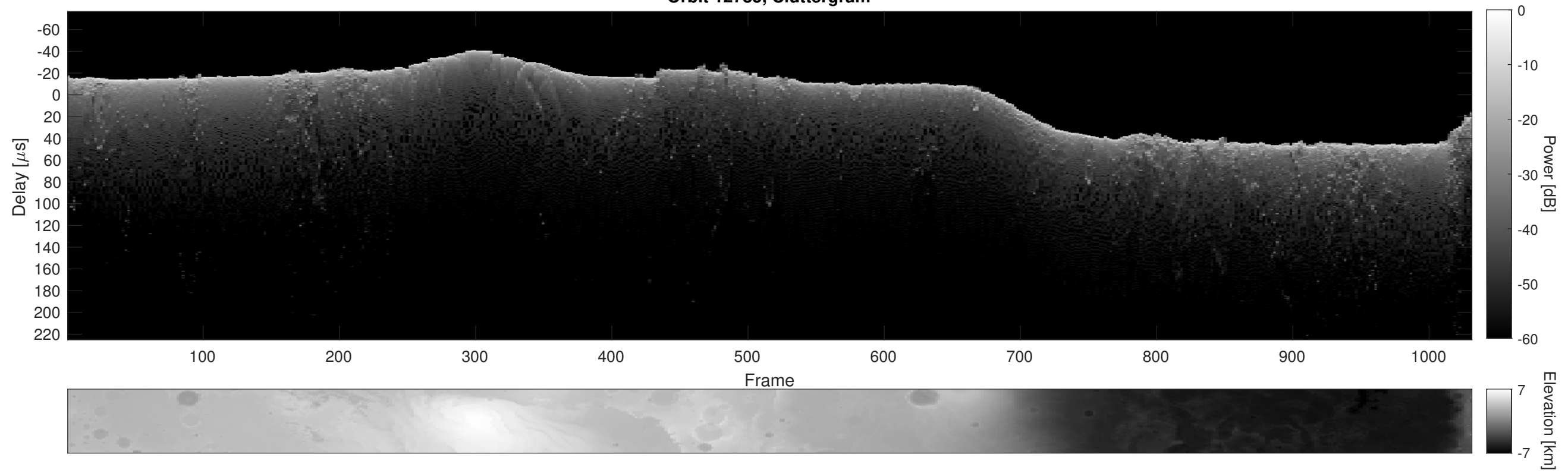
Orbit 12785, Cluttergram
