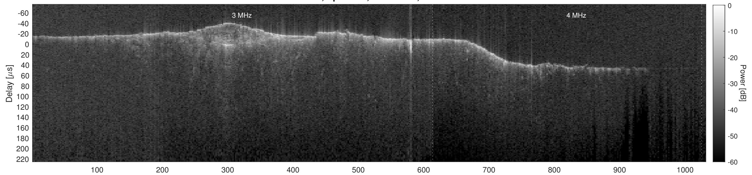
Orbit 12785, Cluttergram
