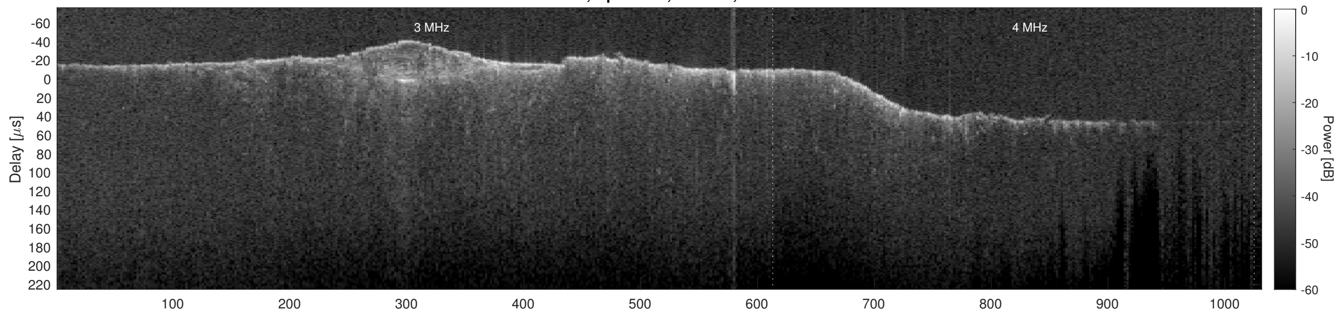
Orbit 12785, Cluttergram
