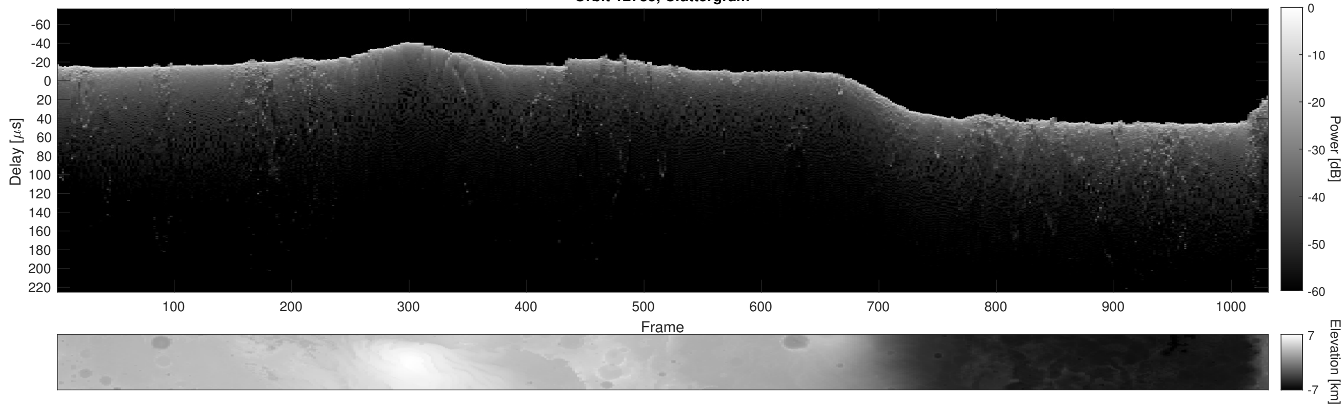
Orbit 12785, Cluttergram
