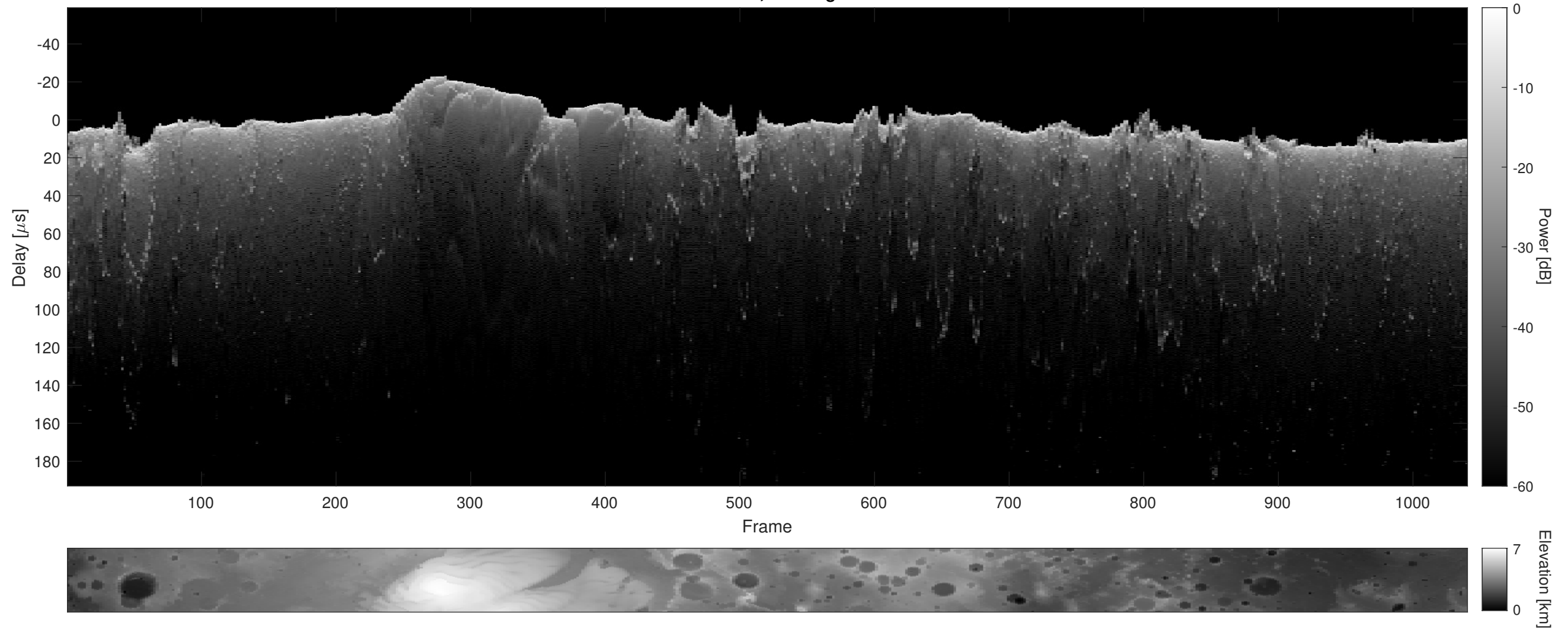
Orbit 12788, Cluttergram
