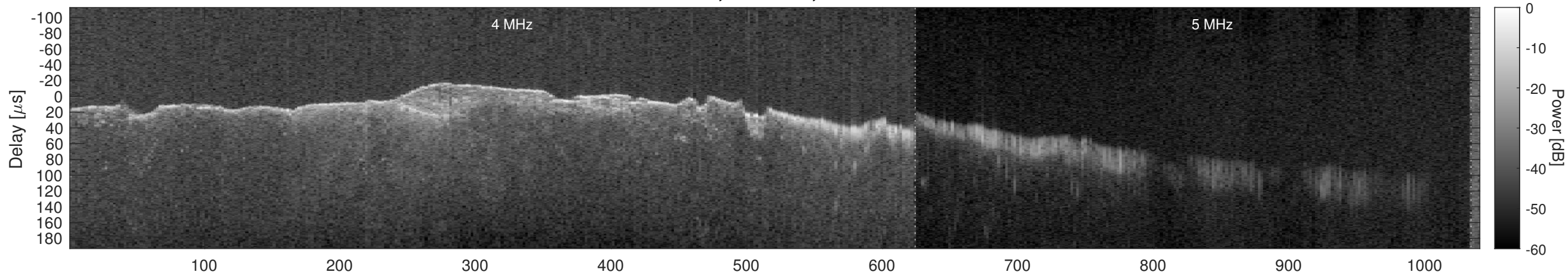
Orbit 12788, Window, Channel 1, Chapman
