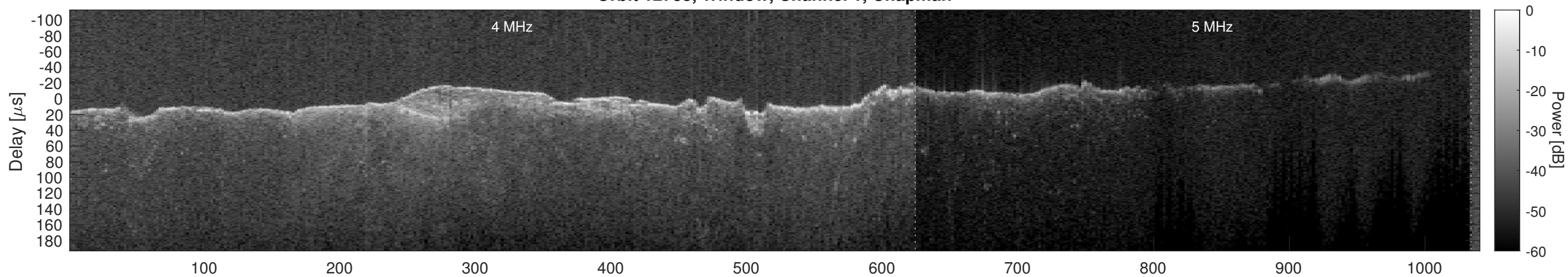
Orbit 12788, Window, Channel 1, Optimized
