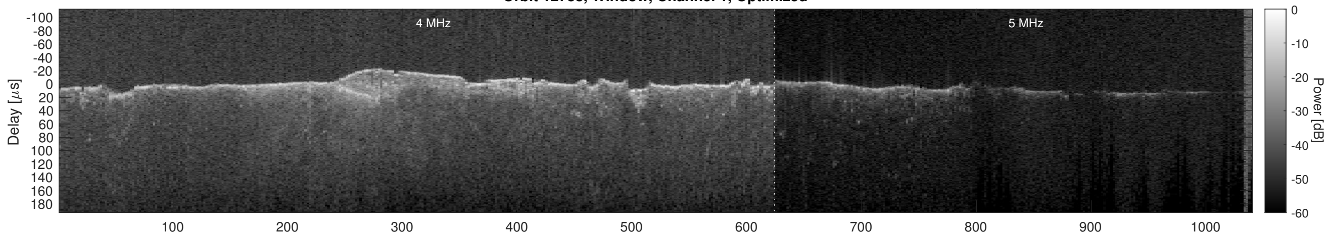
Orbit 12788, Cluttergram
