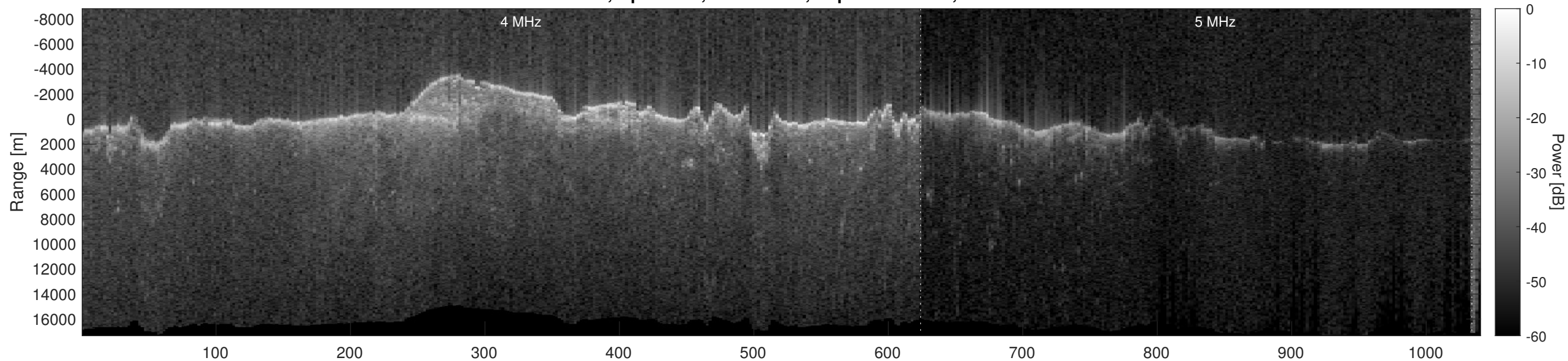
Orbit 12788, Optimized, No Window, Depth-Corrected, Channel 2
