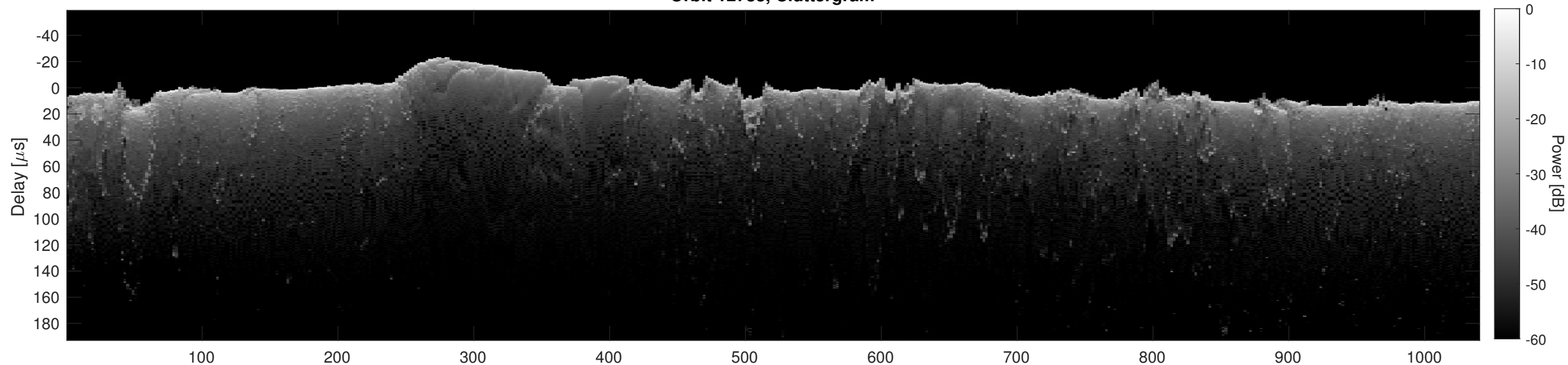
Orbit 12788, Cluttergram
