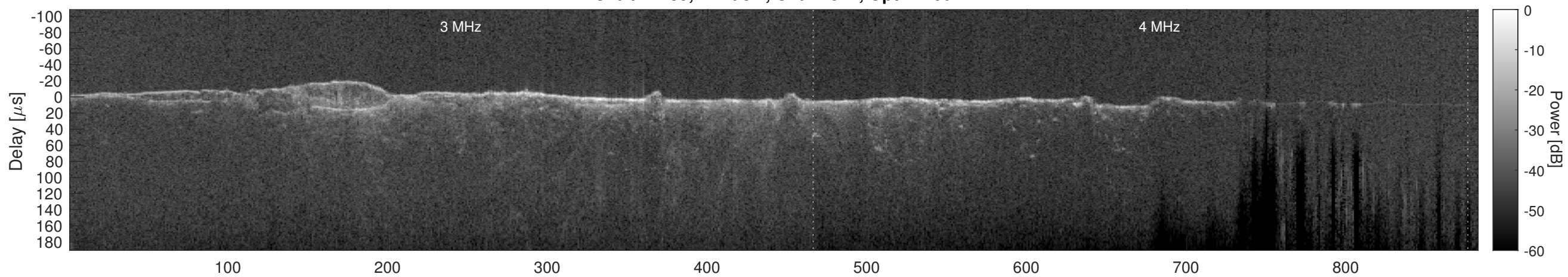
Orbit 12789, Cluttergram
