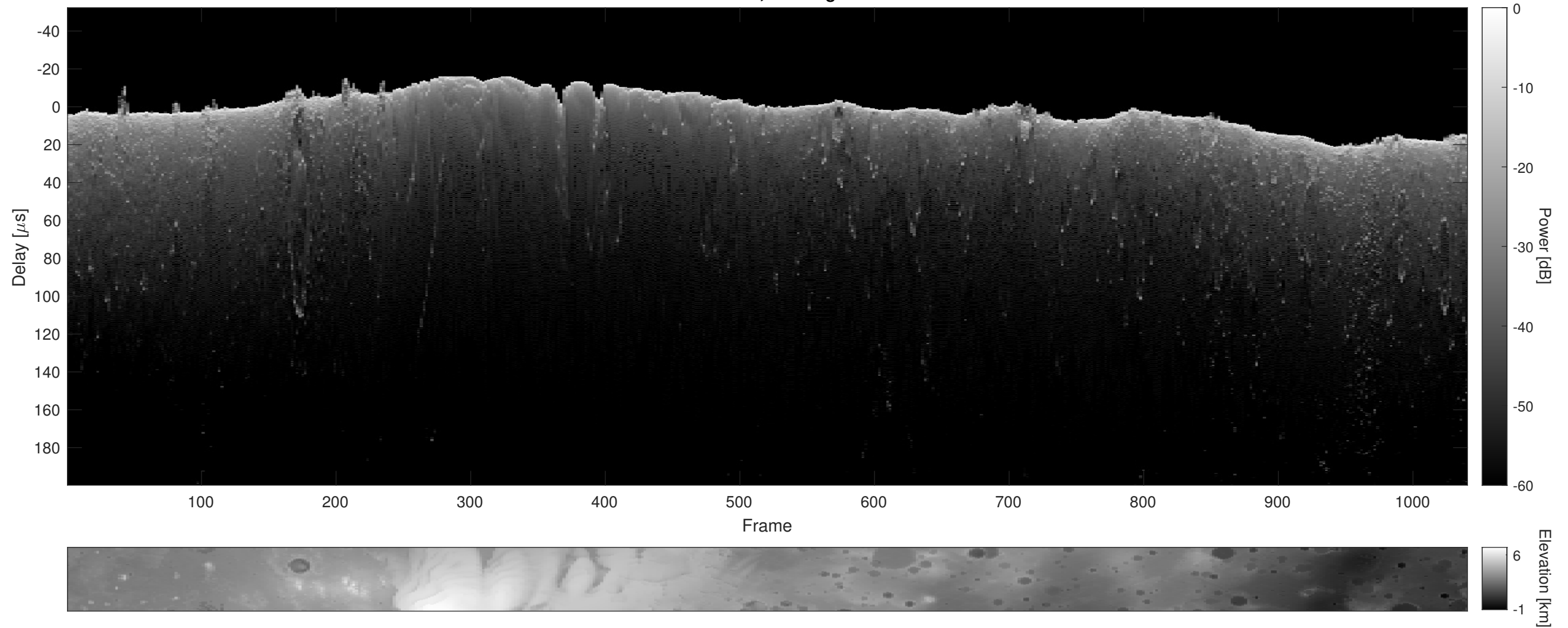
Orbit 12791, Cluttergram
