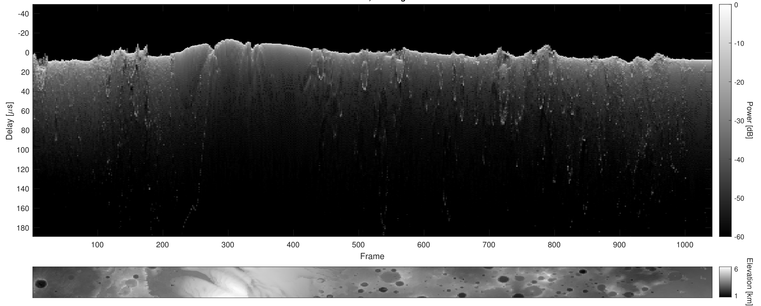
Orbit 12794, Cluttergram
