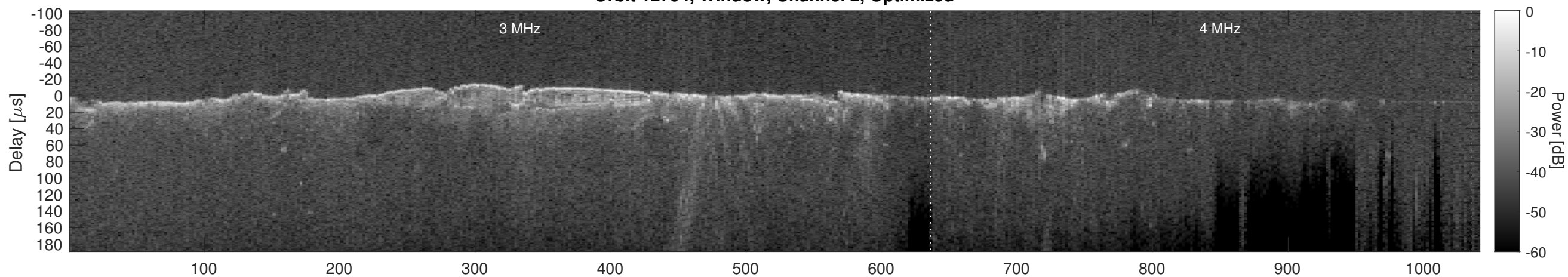
Orbit 12794, Cluttergram
