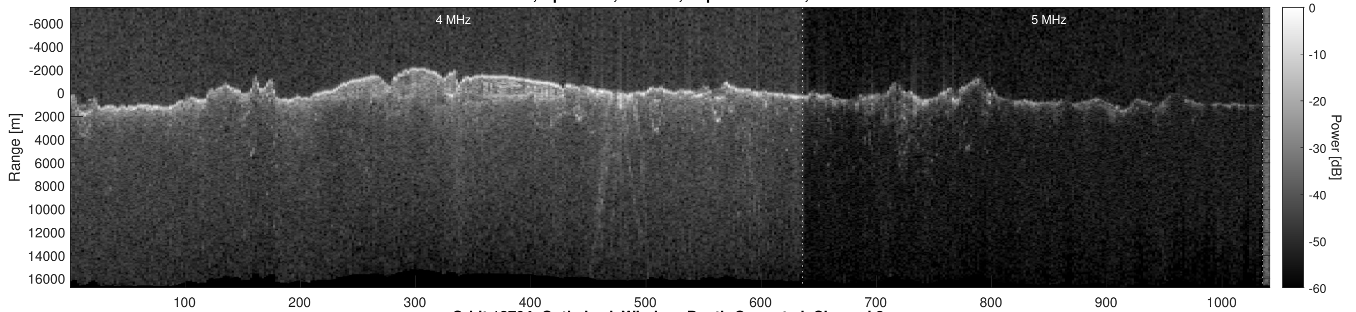
Orbit 12794, Optimized, Window, Depth-Corrected, Channel 2
