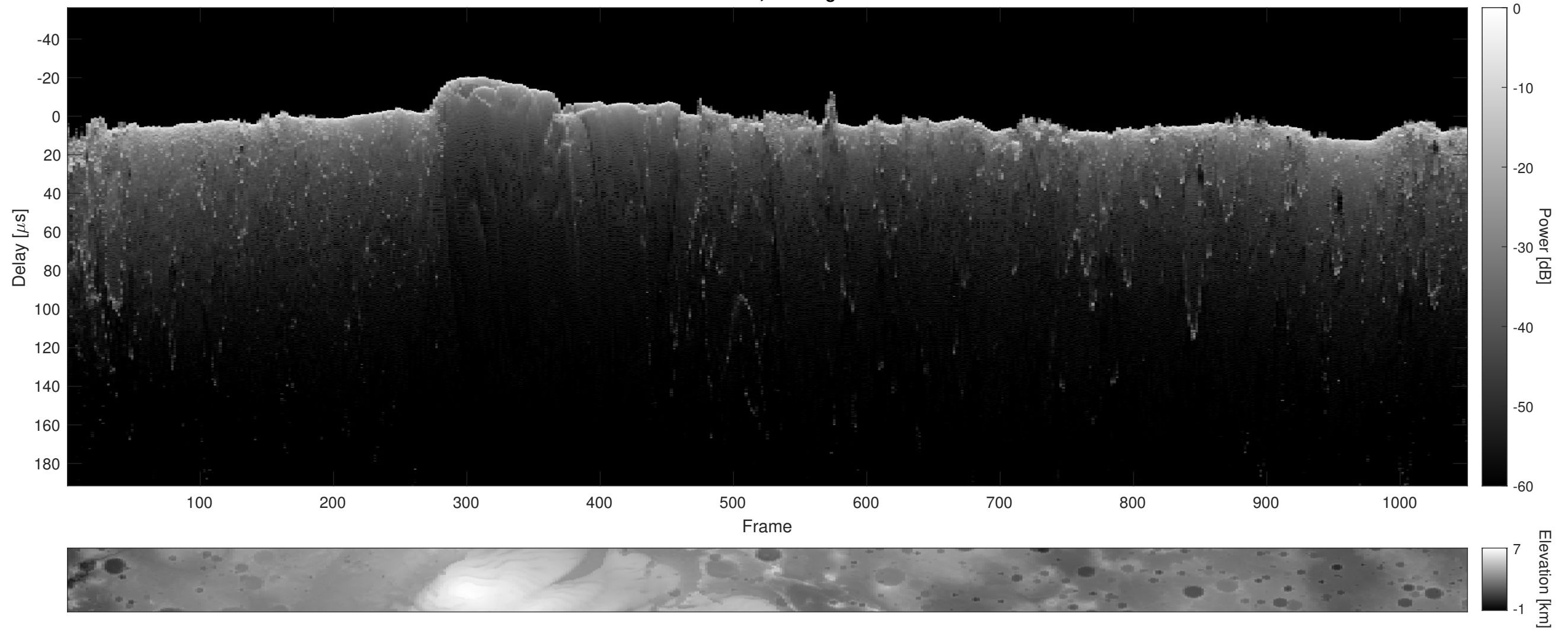
Orbit 12802, Cluttergram
