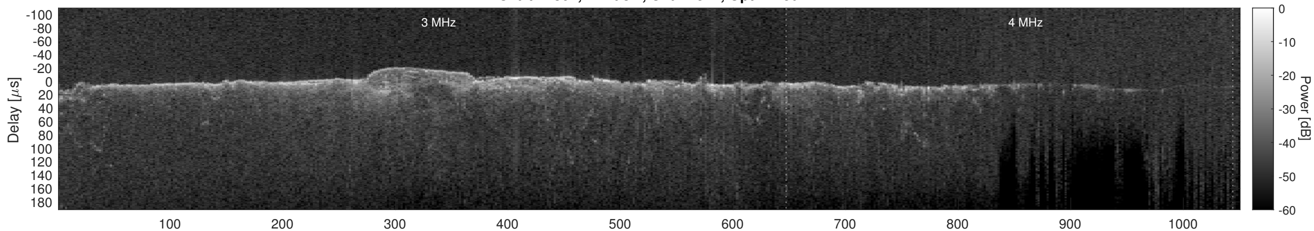
Orbit 12802, Cluttergram
