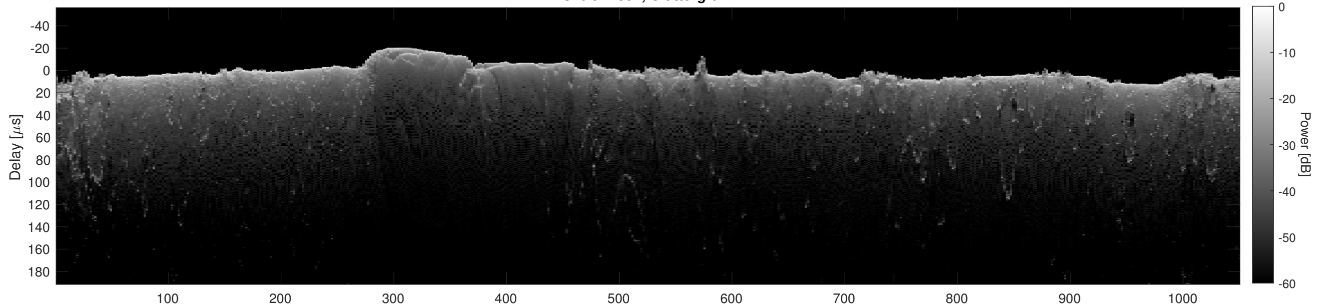
Orbit 12802, Cluttergram
