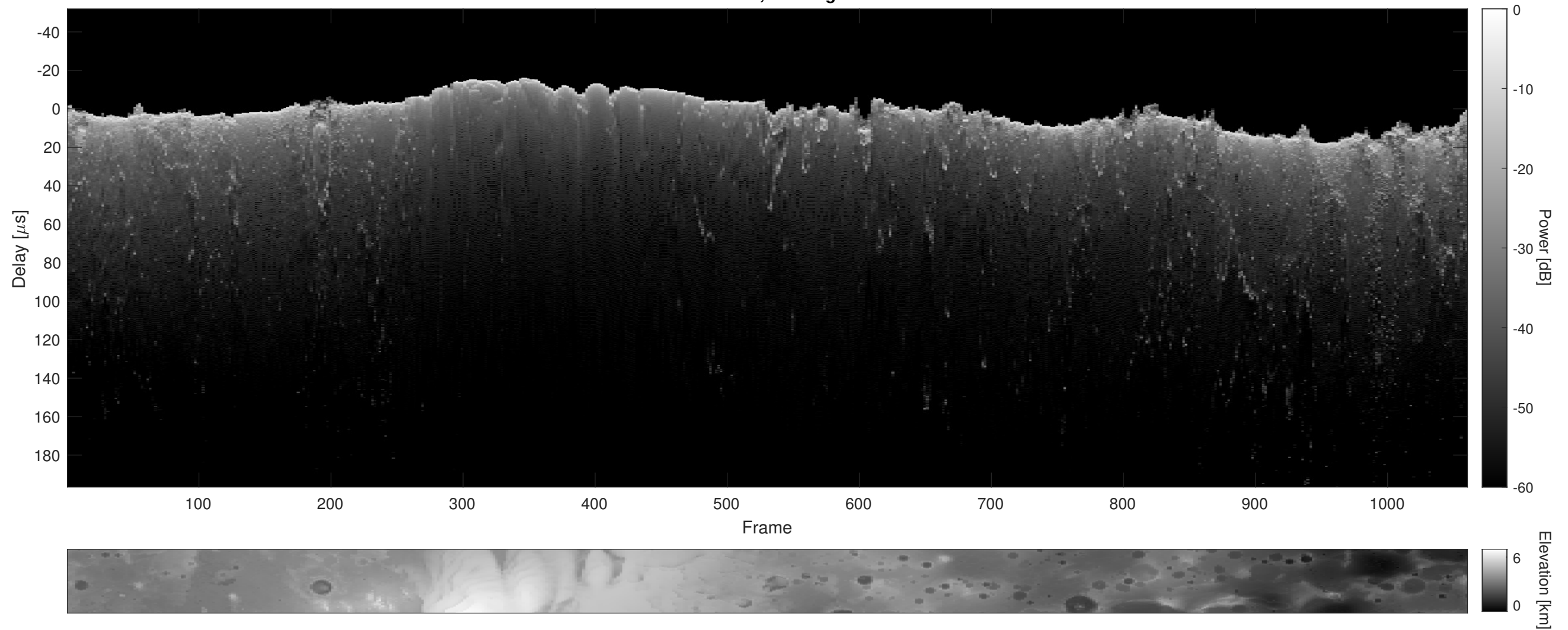
Orbit 12805, Cluttergram
