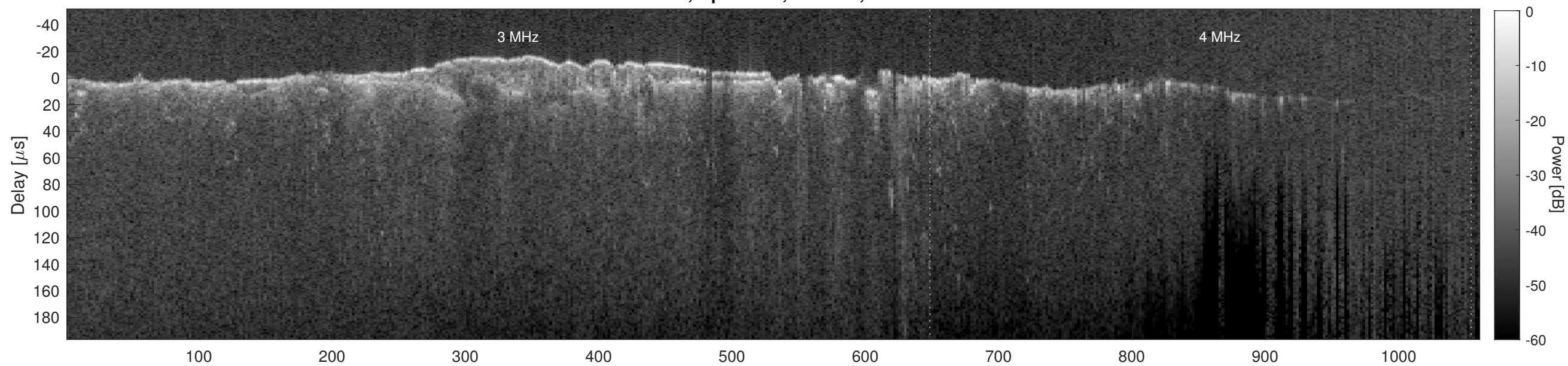
Orbit 12805, Cluttergram
