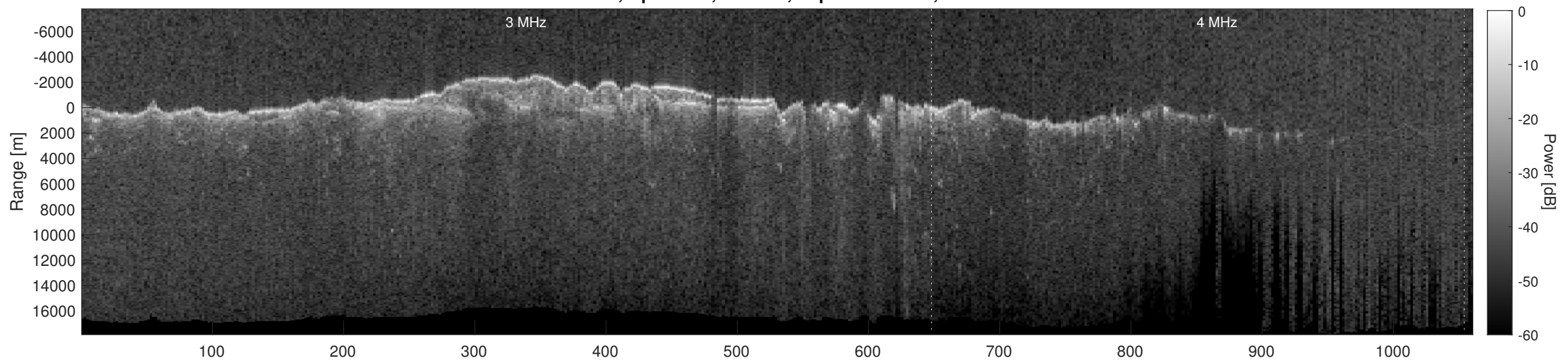
Orbit 12805, Depth-Corrected Cluttergram
