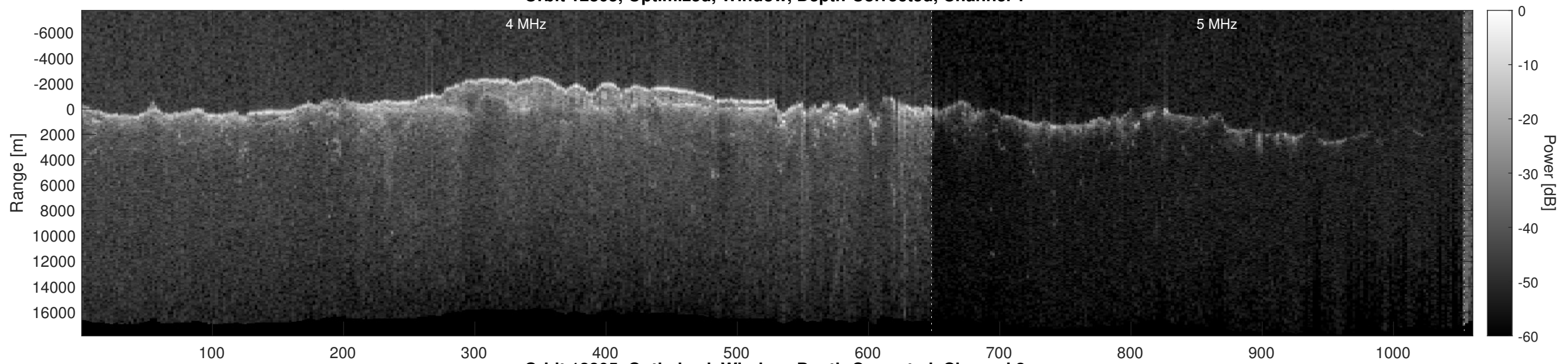
Orbit 12805, Optimized, Window, Depth-Corrected, Channel 2
