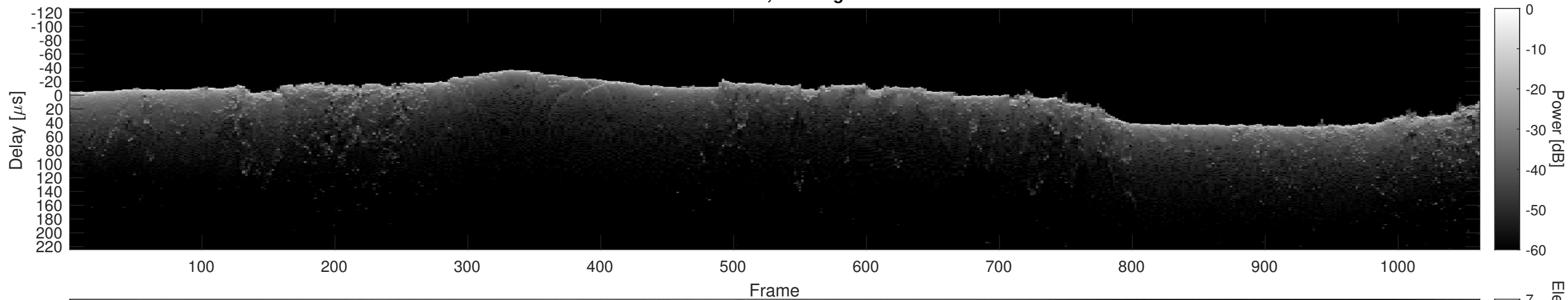
Orbit 12806, Cluttergram
