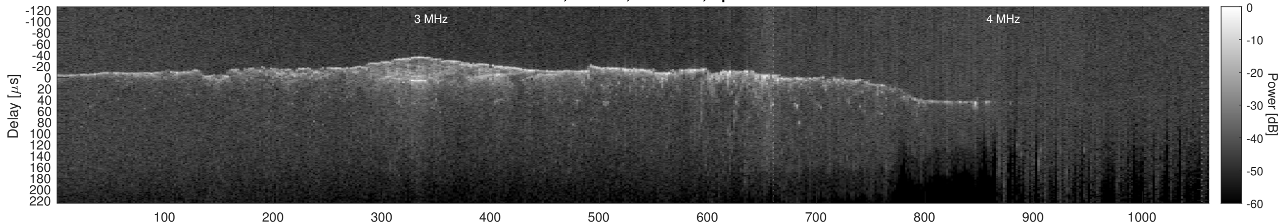
Orbit 12806, Cluttergram
