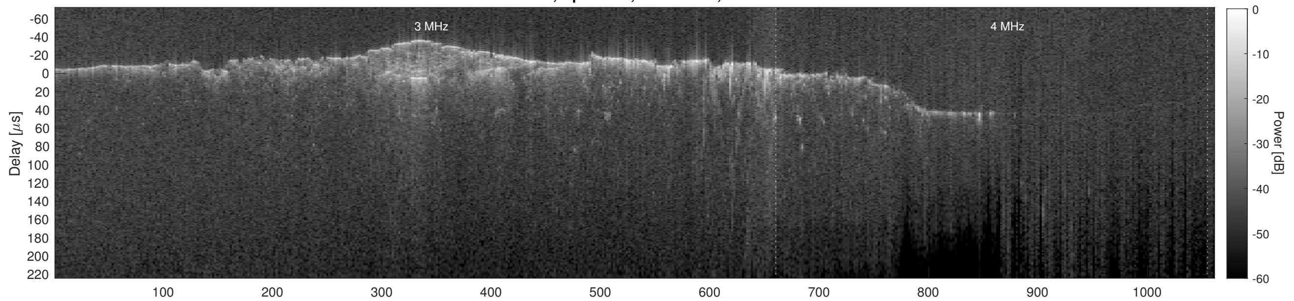
Orbit 12806, Cluttergram
