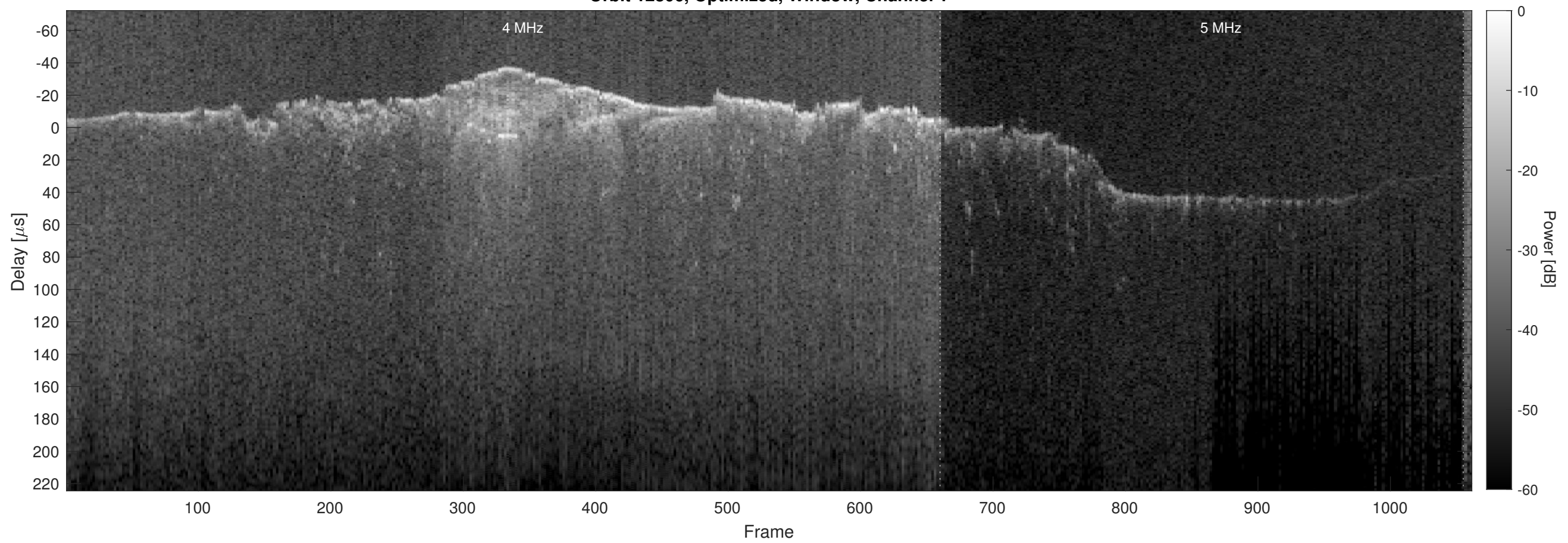
Orbit 12806, Optimized, Window, Channel 2
