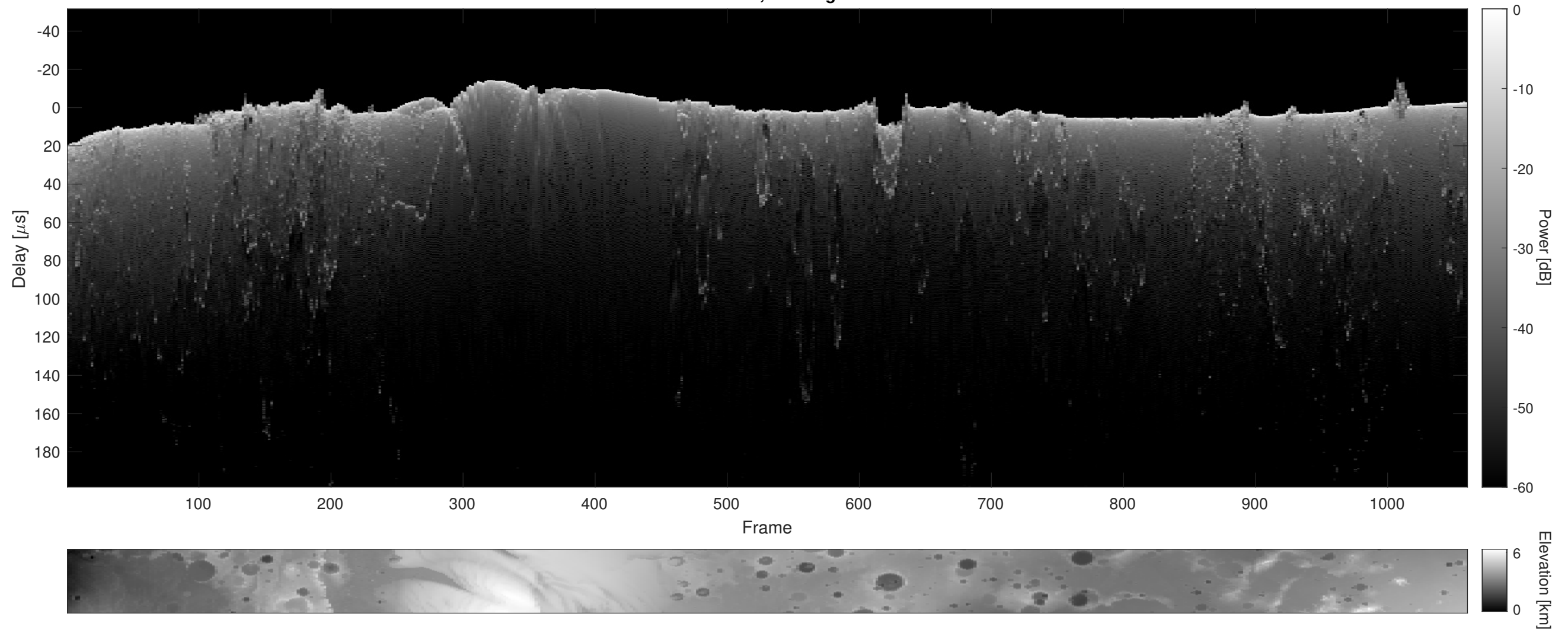
Orbit 12808, Cluttergram
