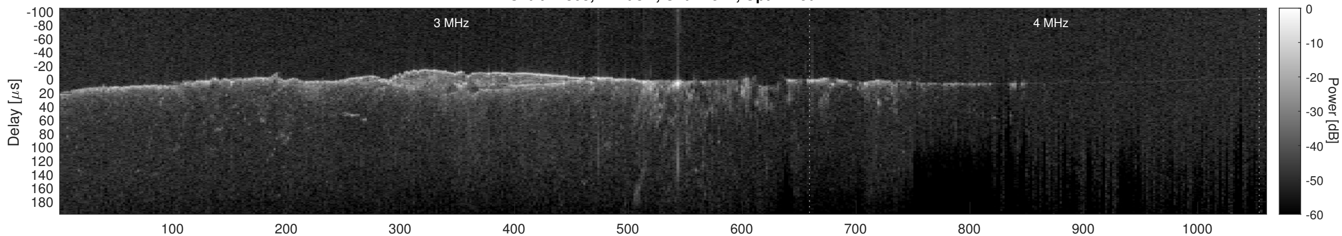
Orbit 12808, Cluttergram
