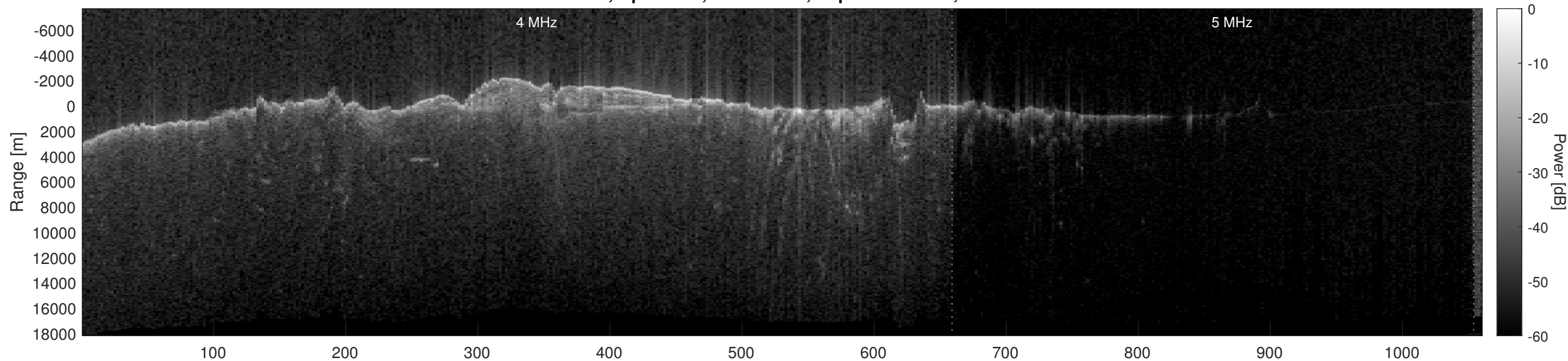
Orbit 12808, Optimized, No Window, Depth-Corrected, Channel 2
