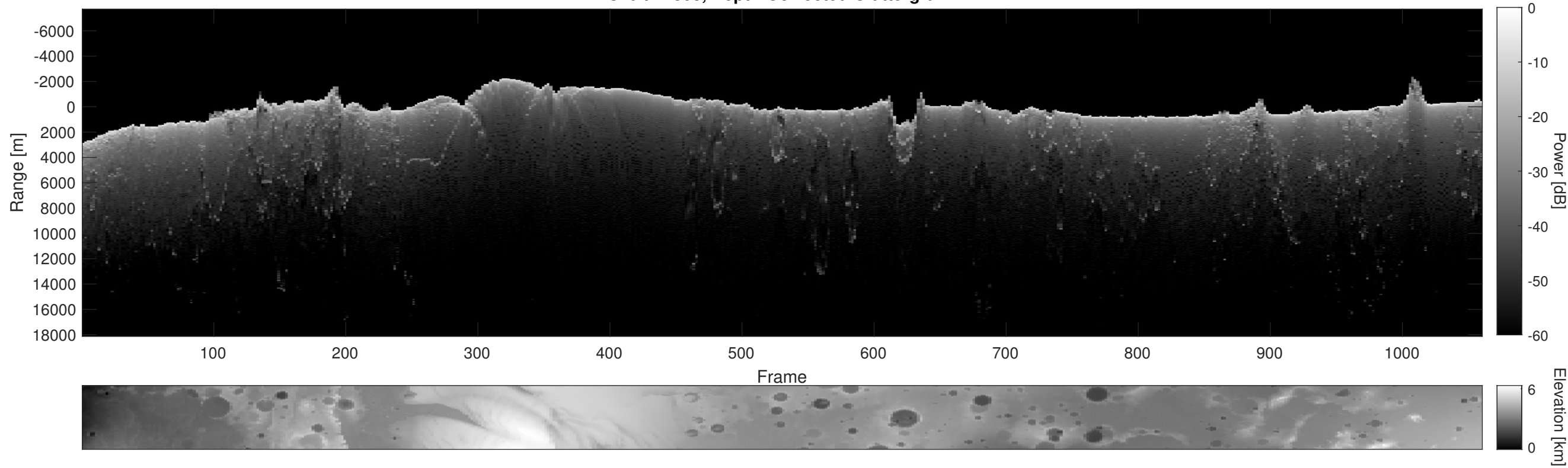
Orbit 12808, Depth-Corrected Cluttergram
