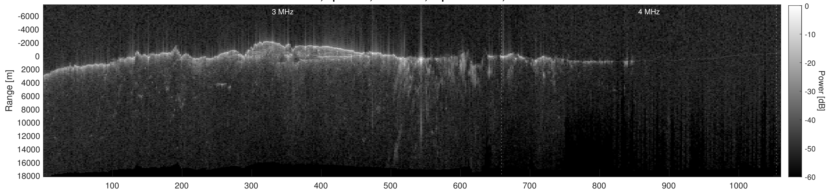
Orbit 12808, Depth-Corrected Cluttergram
