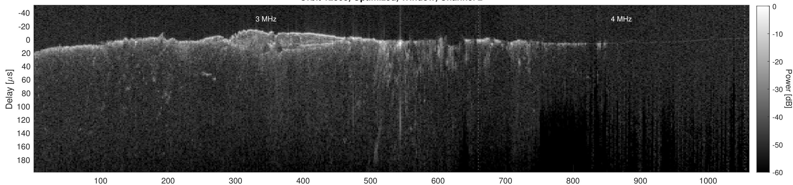
Orbit 12808, Cluttergram
