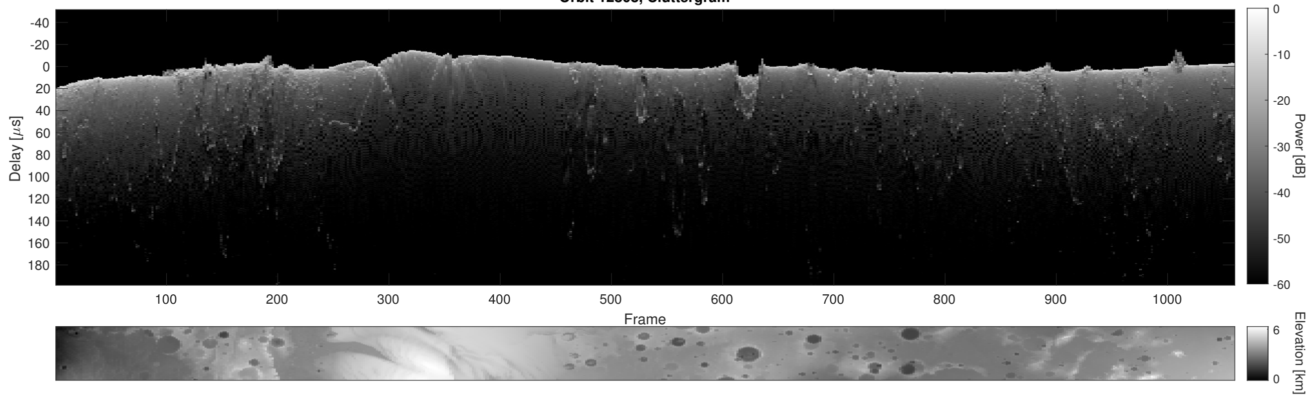
Orbit 12808, Cluttergram
